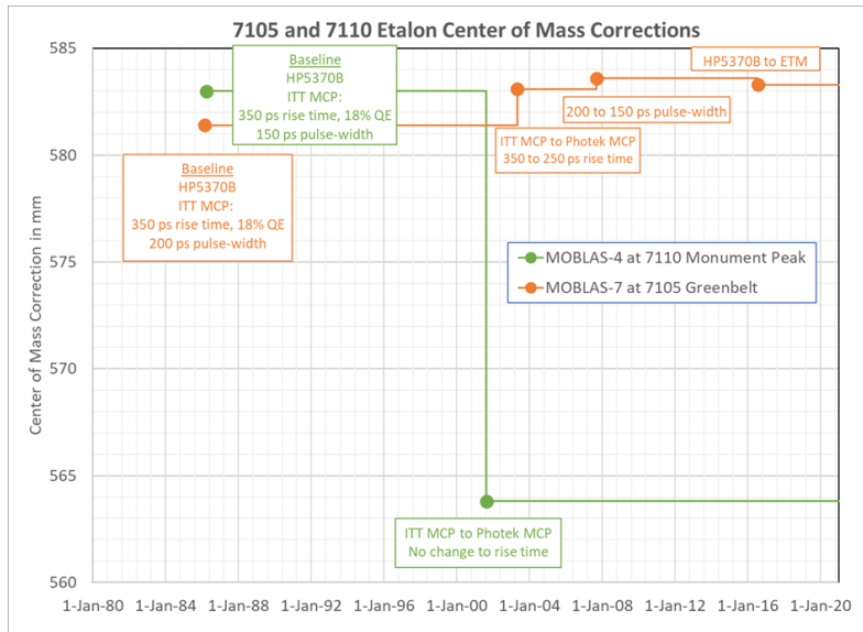
Figure 3: Etalon corrections for MOBLAS stations Goddard and Monument Peak (NASA). The ~2 cm drop for 7110 points to a modelling error. Credit: Van Husson (Peraton).
