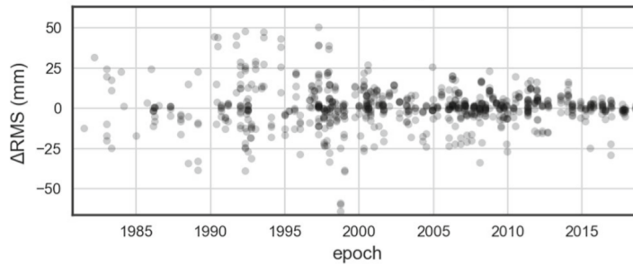
Figure 2: Differences between the modelled and empirical NP RMS for the satellites and stations included in the first release of the CoM tables [1].
