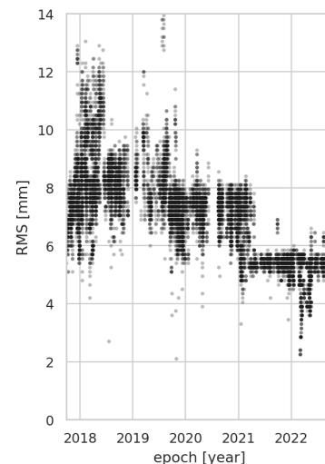
Figure 4: RMS of normal points from 7821.
