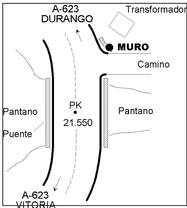
Muro Km. 21,550
