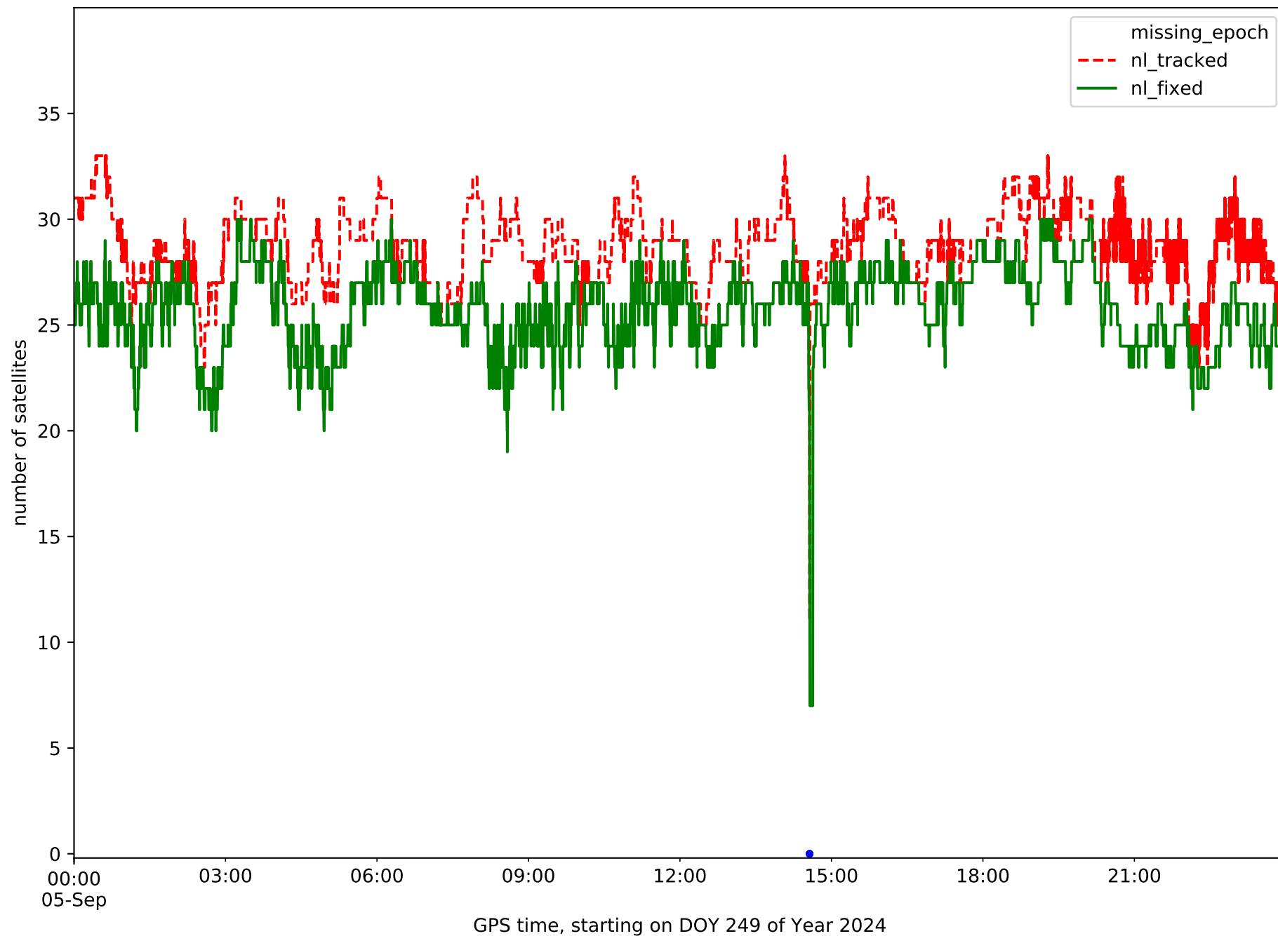
Station MENC in network NT11
