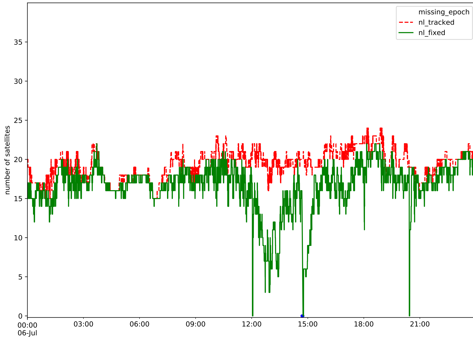
GPS time, starting on DOY 188 of Year 2024
