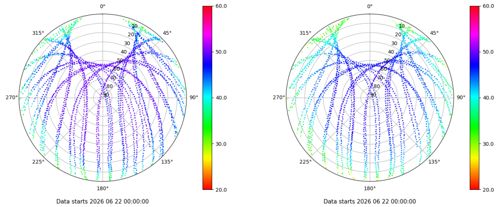
Skyplot for station ZFRA. Signal to Noise S1C Data file ZFRA00ESP_R_2026173.xtr Skyplot for station ZFRA. Signal to Noise S2P Data file ZFRA00ESP_R_2026173.xtr
