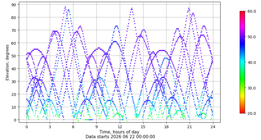
Time-elevation plot for station ZFRA. Signal to Noise S1C Data file ZFRA00ESP_R_2026173.xtr
