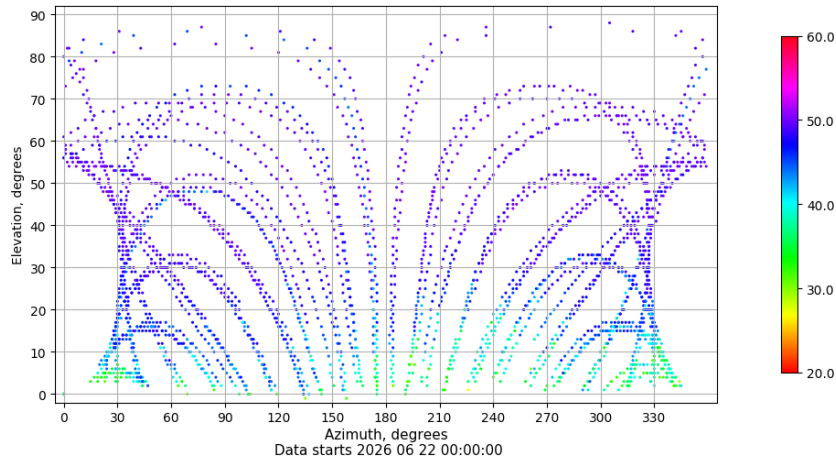
Azimuth-elevation plot for station ZFRA. Signal to Noise S1C Data file ZFRA00ESP_R_2026173.xtr
