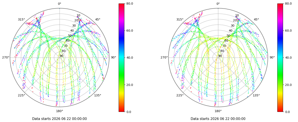
Skyplot for station ZFRA. Parameter M1C Data file ZFRA00ESP_R_2026173.xtr Skyplot for station ZFRA. Parameter M2P Data file ZFRA00ESP_R_2026173.xtr
