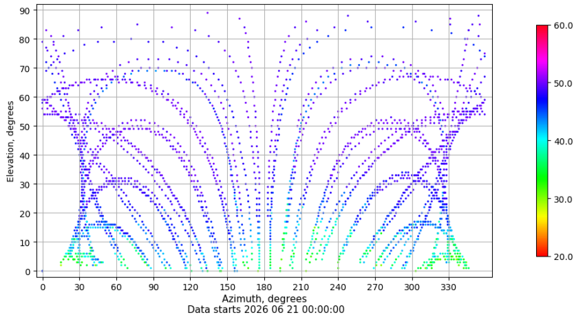
Azimuth-elevation plot for station ZFRA. Signal to Noise S1C Data file ZFRA00ESP_R_2026172.xtr
