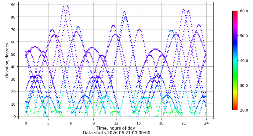
Time-elevation plot for station ZFRA. Signal to Noise S1C Data file ZFRA00ESP_R_2026172.xtr
