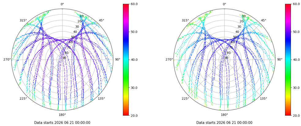
Skyplot for station ZFRA. Signal to Noise S1C Data file ZFRA00ESP_R_2026172.xtr Skyplot for station ZFRA. Signal to Noise S2P Data file ZFRA00ESP_R_2026172.xtr
