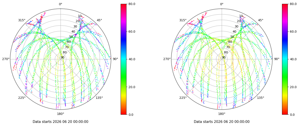
Skyplot for station ZFRA. Parameter M1C Data file ZFRA00ESP_R_2026171.xtr Skyplot for station ZFRA. Parameter M2P Data file ZFRA00ESP_R_2026171.xtr
