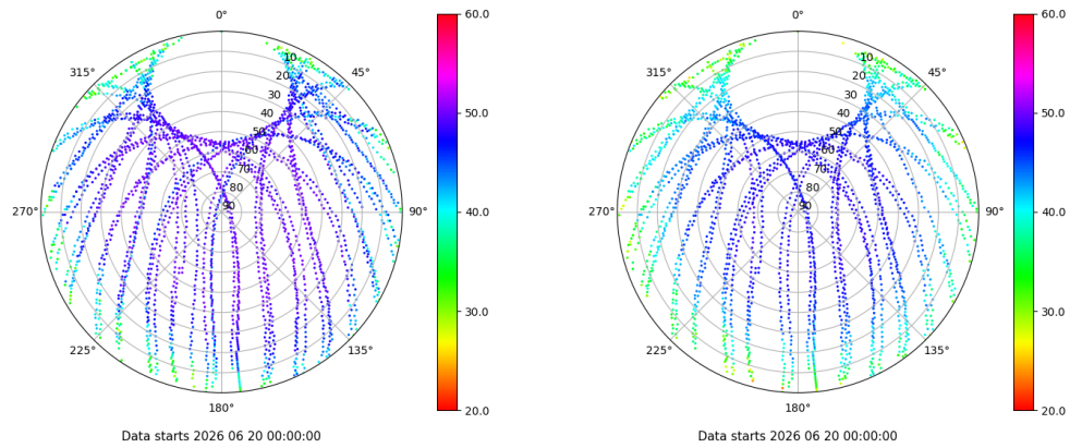
Skyplot for station ZFRA. Signal to Noise S1C Data file ZFRA00ESP_R_2026171.xtr Skyplot for station ZFRA. Signal to Noise S2P Data file ZFRA00ESP_R_2026171.xtr
