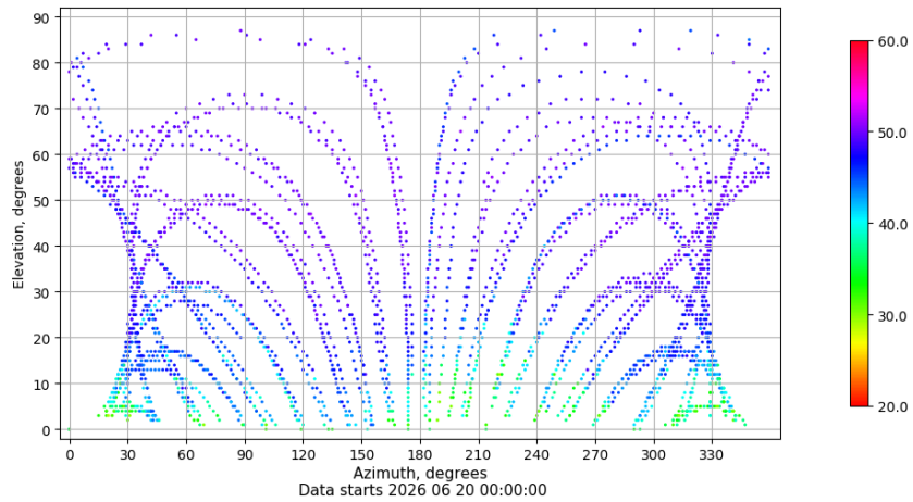
Azimuth-elevation plot for station ZFRA. Signal to Noise S1C Data file ZFRA00ESP_R_2026171.xtr
