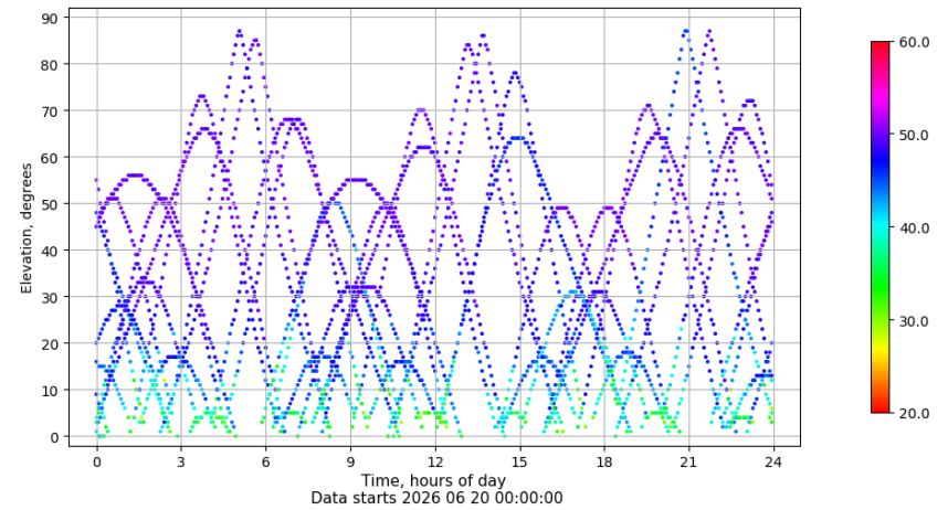
Time-elevation plot for station ZFRA. Signal to Noise S1C Data file ZFRA00ESP_R_2026171.xtr
