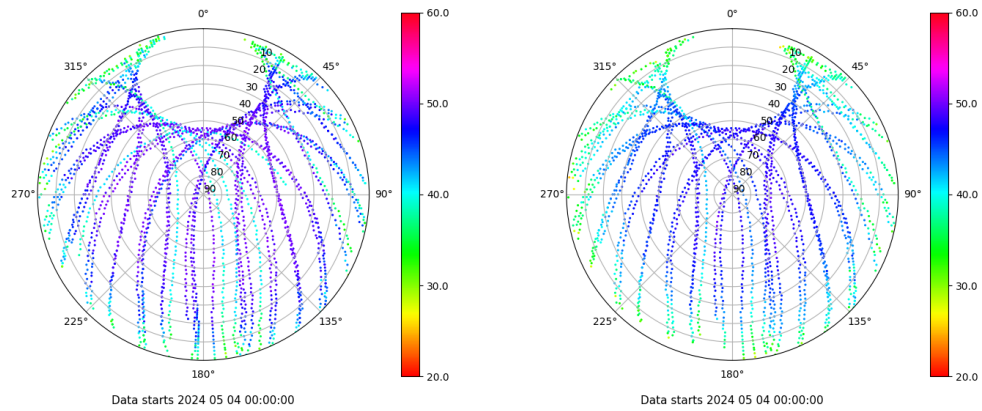
Skyplot for station ZFRA. Signal to Noise S1C Data file ZFRA00ESP_R_2024125.xtr Skyplot for station ZFRA. Signal to Noise S2P Data file ZFRA00ESP_R_2024125.xtr
