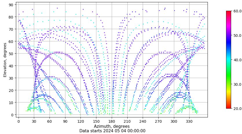
Azimuth-elevation plot for station ZFRA. Signal to Noise S1C Data file ZFRA00ESP_R_2024125.xtr
