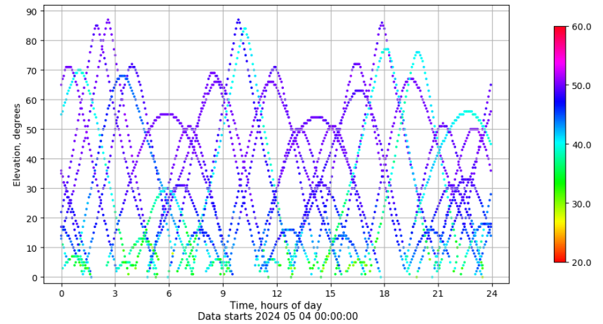
Time-elevation plot for station ZFRA. Signal to Noise S1C Data file ZFRA00ESP_R_2024125.xtr
