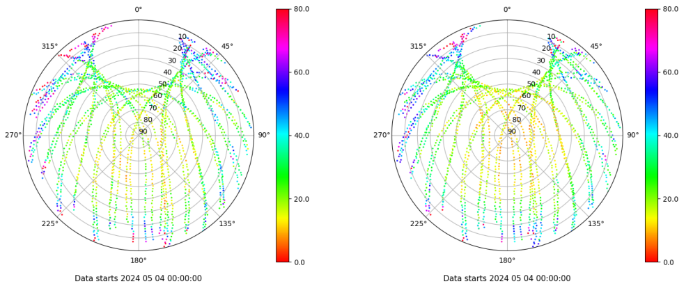
Skyplot for station ZFRA. Parameter M1C Data file ZFRA00ESP_R_2024125.xtr Skyplot for station ZFRA. Parameter M2P Data file ZFRA00ESP_R_2024125.xtr
