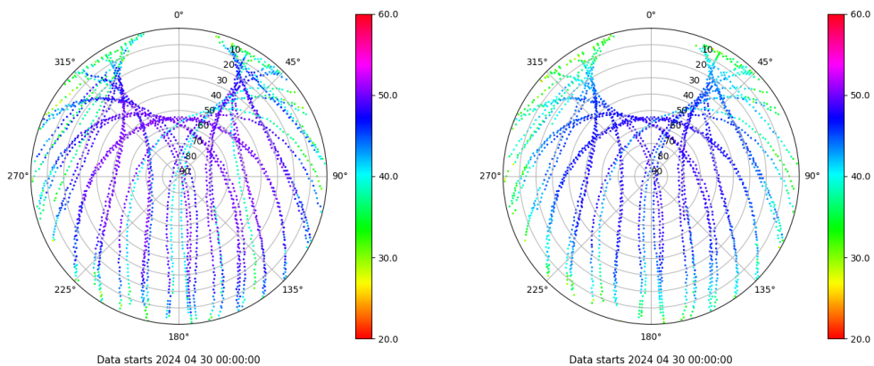
Skyplot for station ZFRA. Signal to Noise S1C Data file ZFRA00ESP_R_2024121.xtr Skyplot for station ZFRA. Signal to Noise S2P Data file ZFRA00ESP_R_2024121.xtr
