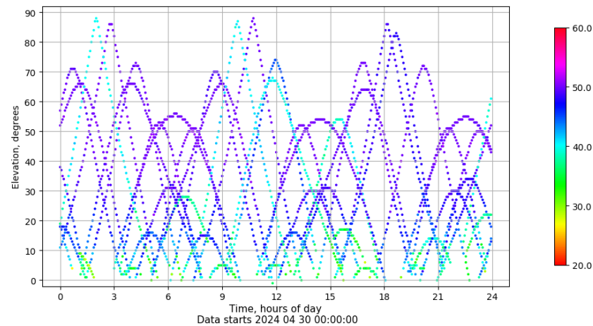
Time-elevation plot for station ZFRA. Signal to Noise S1C Data file ZFRA00ESP_R_2024121.xtr
