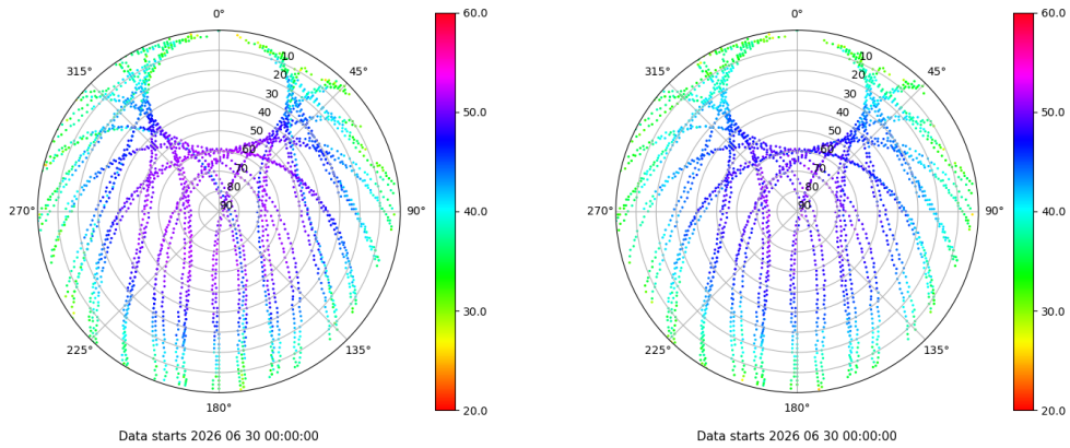
Skyplot for station VIGO. Signal to Noise S1C Data file VIGO00ESP_R_2026181.xtr Skyplot for station VIGO. Signal to Noise S2C Data file VIGO00ESP_R_2026181.xtr
