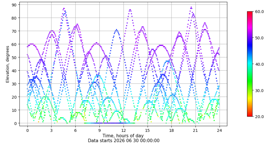
Time-elevation plot for station VIGO. Signal to Noise S1C Data file VIGO00ESP_R_2026181.xtr
