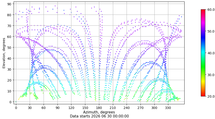
Azimuth-elevation plot for station VIGO. Signal to Noise S1C Data file VIGO00ESP_R_2026181.xtr
