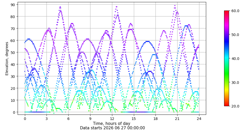
Time-elevation plot for station VIGO. Signal to Noise S1C Data file VIGO00ESP_R_2026178.xtr
