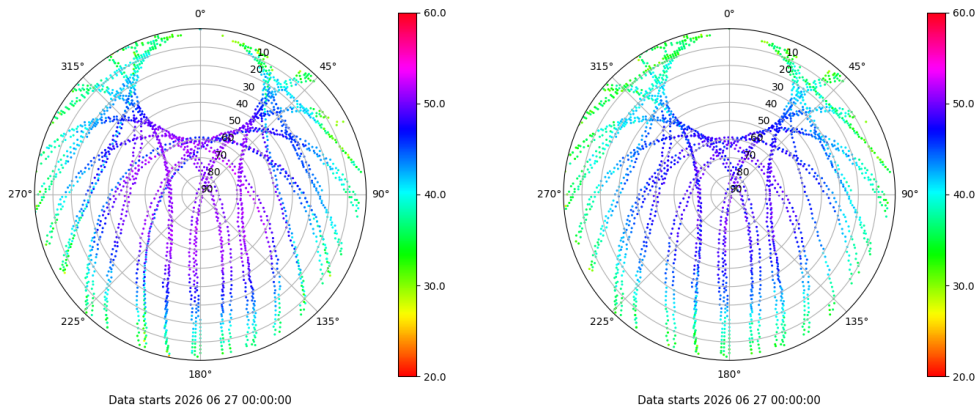
Skyplot for station VIGO. Signal to Noise S1C Data file VIGO00ESP_R_2026178.xtr Skyplot for station VIGO. Signal to Noise S2C Data file VIGO00ESP_R_2026178.xtr
