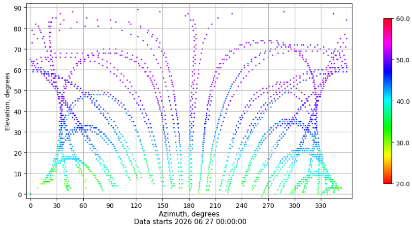
Azimuth-elevation plot for station VIGO. Signal to Noise S1C Data file VIGO00ESP_R_2026178.xtr
