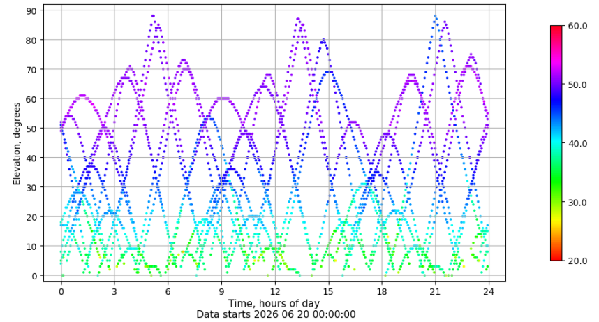
Time-elevation plot for station VIGO. Signal to Noise S1C Data file VIGO00ESP_R_2026171.xtr
