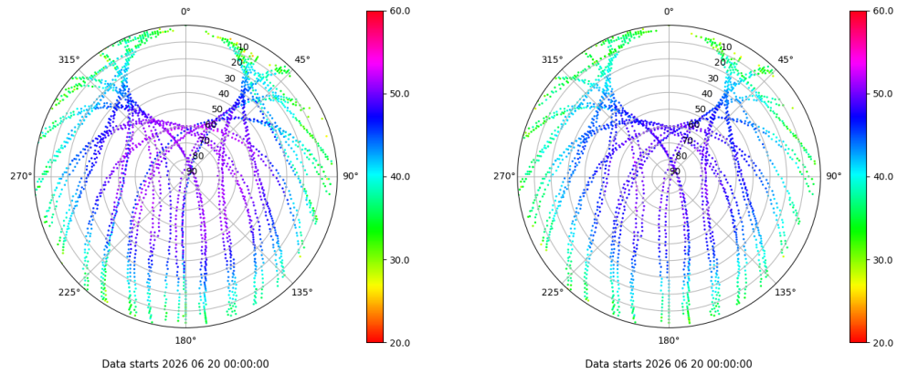
Skyplot for station VIGO. Signal to Noise S1C Data file VIGO00ESP_R_2026171.xtr Skyplot for station VIGO. Signal to Noise S2C Data file VIGO00ESP_R_2026171.xtr
