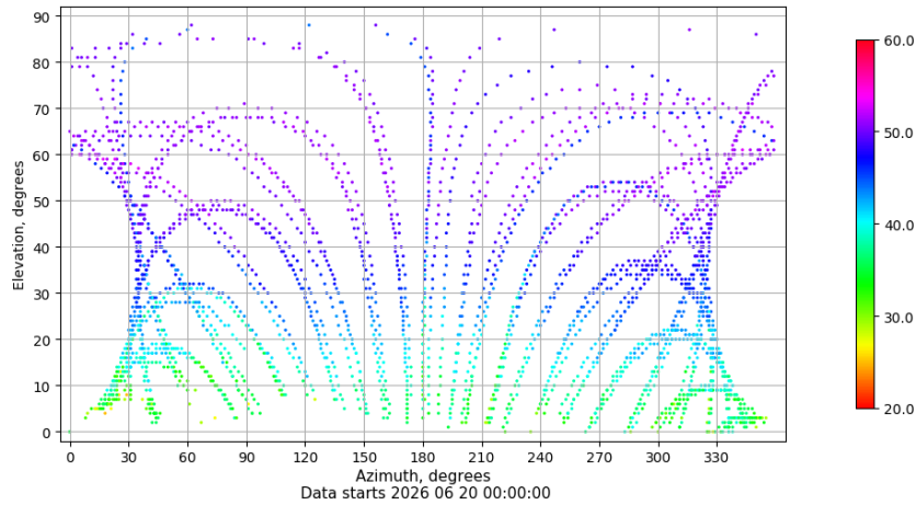
Azimuth-elevation plot for station VIGO. Signal to Noise S1C Data file VIGO00ESP_R_2026171.xtr
