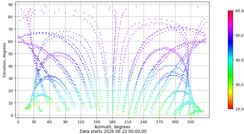
Azimuth-elevation plot for station VIGO. Signal to Noise S1C Data file VIGO00ESP_R_2026161.xtr
