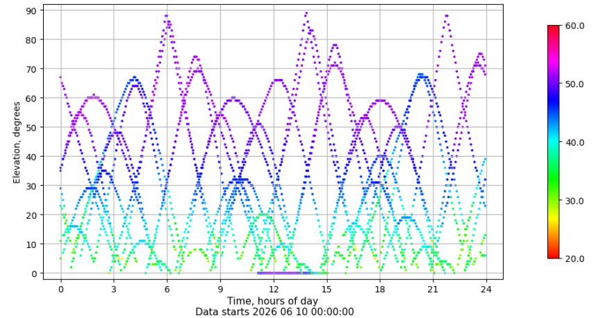
Time-elevation plot for station VIGO. Signal to Noise S1C Data file VIGO00ESP_R_2026161.xtr
