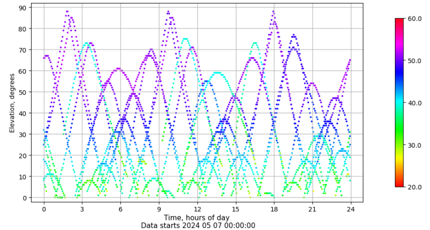
Time-elevation plot for station VIGO. Signal to Noise S1C Data file VIGO00ESP_R_2024128.xtr
