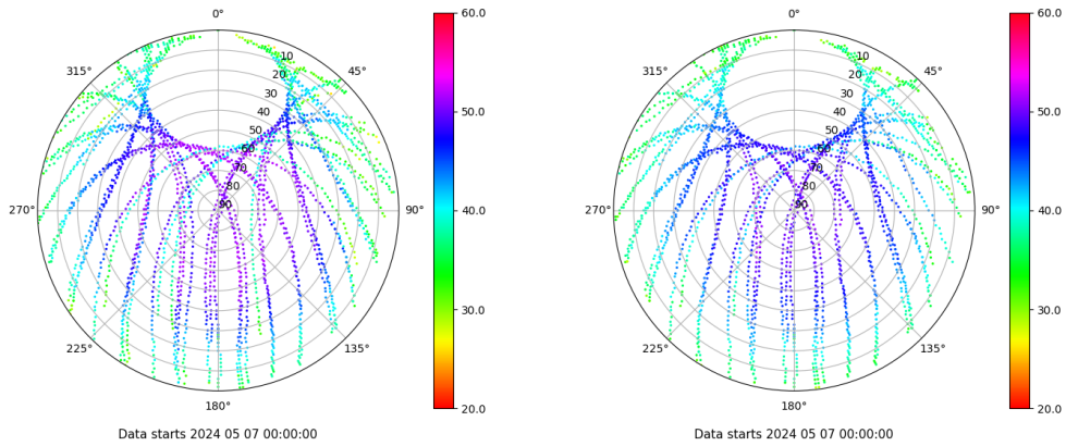
Skyplot for station VIGO. Signal to Noise S1C Data file VIGO00ESP_R_2024128.xtr Skyplot for station VIGO. Signal to Noise S2C Data file VIGO00ESP_R_2024128.xtr
