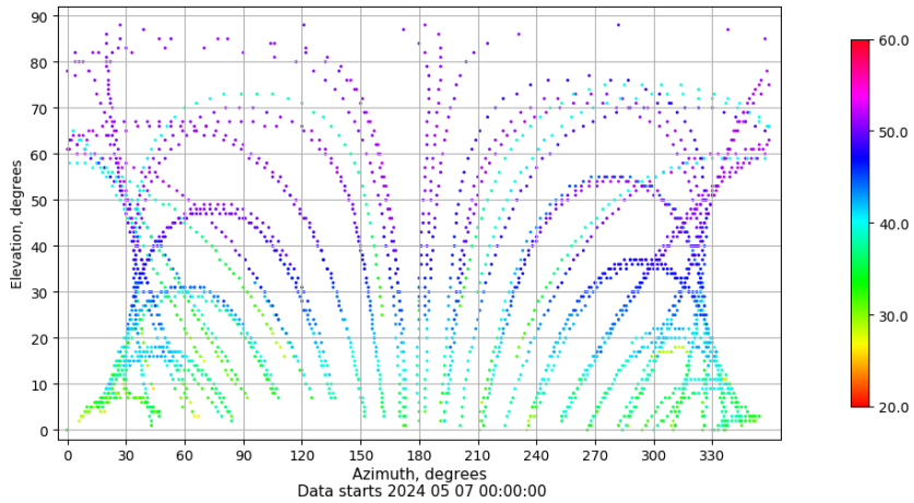
Azimuth-elevation plot for station VIGO. Signal to Noise S1C Data file VIGO00ESP_R_2024128.xtr
