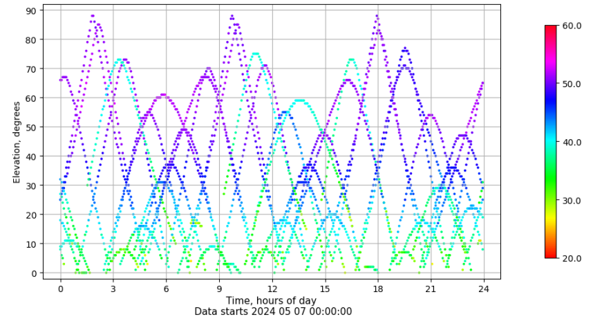
Time-elevation plot for station VIGO. Signal to Noise S1C Data file VIGO00ESP_R_2024128.xtr
