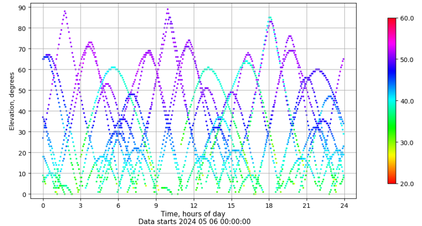
Time-elevation plot for station VIGO. Signal to Noise S1C Data file VIGO00ESP_R_2024127.xtr
