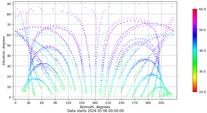
Azimuth-elevation plot for station VIGO. Signal to Noise S1C Data file VIGO00ESP_R_2024127.xtr
