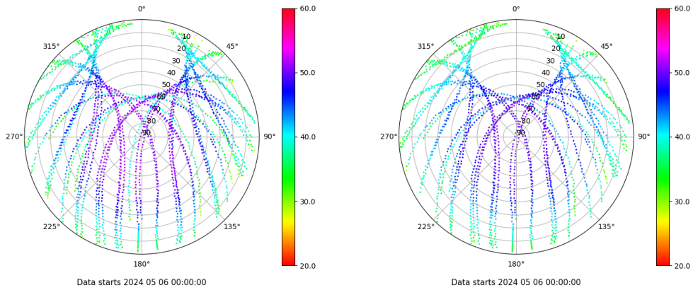
Skyplot for station VIGO. Signal to Noise S1C Data file VIGO00ESP_R_2024127.xtr Skyplot for station VIGO. Signal to Noise S2C Data file VIGO00ESP_R_2024127.xtr
