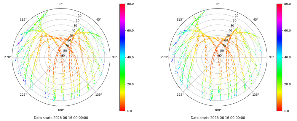
Skyplot for station VICA. Parameter M1C Data file VICA00ESP_R_2026167.xtr Skyplot for station VICA. Parameter M2P Data file VICA00ESP_R_2026167.xtr
