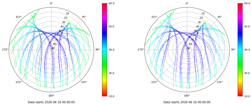
Skyplot for station VICA. Signal to Noise S1C Data file VICA00ESP_R_2026167.xtr Skyplot for station VICA. Signal to Noise S2P Data file VICA00ESP_R_2026167.xtr
