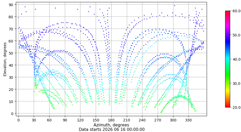
Azimuth-elevation plot for station VICA. Signal to Noise S1C Data file VICA00ESP_R_2026167.xtr
