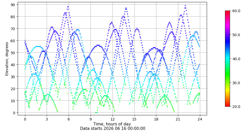
Time-elevation plot for station VICA. Signal to Noise S1C Data file VICA00ESP_R_2026167.xtr
