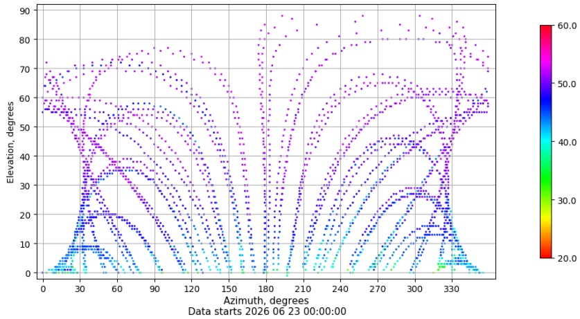
Azimuth-elevation plot for station VALE. Signal to Noise S1C Data file VALE00ESP_R_2026174.xtr
