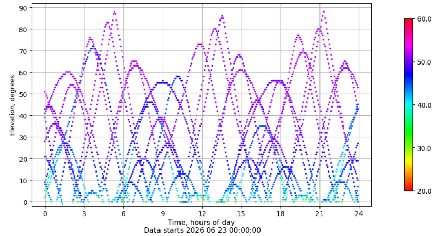
Time-elevation plot for station VALE. Signal to Noise S1C Data file VALE00ESP_R_2026174.xtr
