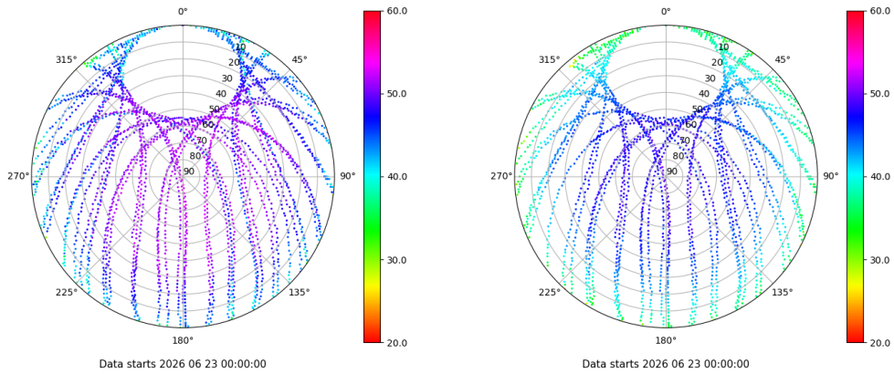
Skyplot for station VALE. Signal to Noise S1C Data file VALE00ESP_R_2026174.xtr Skyplot for station VALE. Signal to Noise S2P Data file VALE00ESP_R_2026174.xtr
