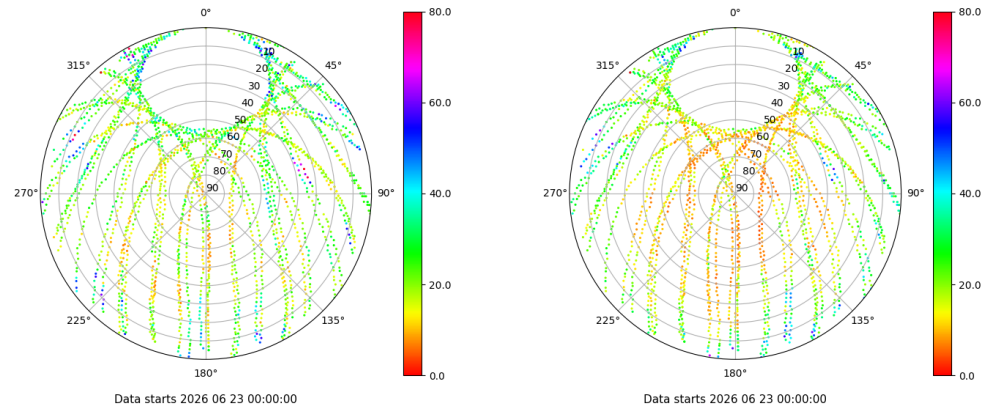
Skyplot for station VALE. Parameter M1C Data file VALE00ESP_R_2026174.xtr Skyplot for station VALE. Parameter M2P Data file VALE00ESP_R_2026174.xtr
