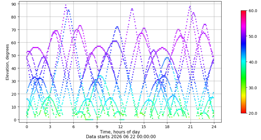
Time-elevation plot for station VALC. Signal to Noise S1C Data file VALC00ESP_R_2026173.xtr
