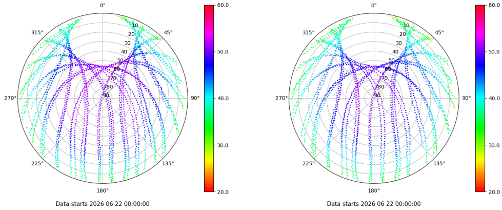
Skyplot for station VALC. Signal to Noise S1C Data file VALC00ESP_R_2026173.xtr Skyplot for station VALC. Signal to Noise S2C Data file VALC00ESP_R_2026173.xtr
