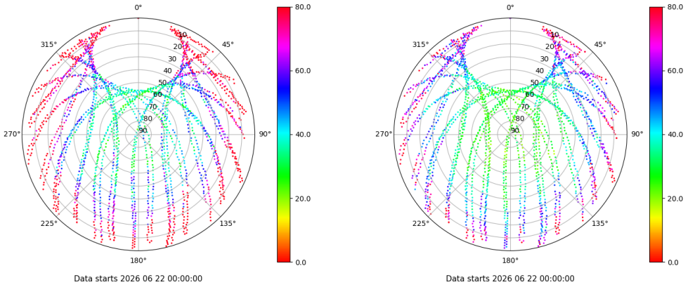
Skyplot for station VALC. Parameter M1C Data file VALC00ESP_R_2026173.xtr Skyplot for station VALC. Parameter M2C Data file VALC00ESP_R_2026173.xtr
