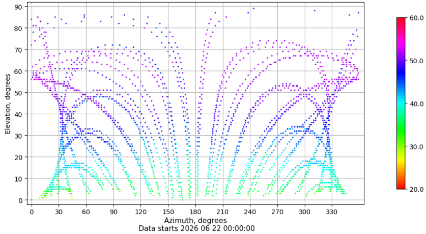
Azimuth-elevation plot for station VALC. Signal to Noise S1C Data file VALC00ESP_R_2026173.xtr
