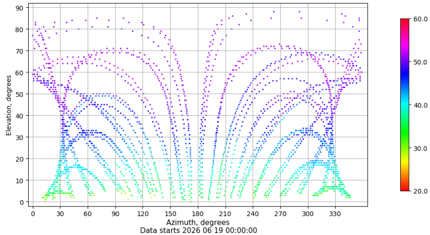
Azimuth-elevation plot for station VALC. Signal to Noise S1C Data file VALC00ESP_R_2026170.xtr
