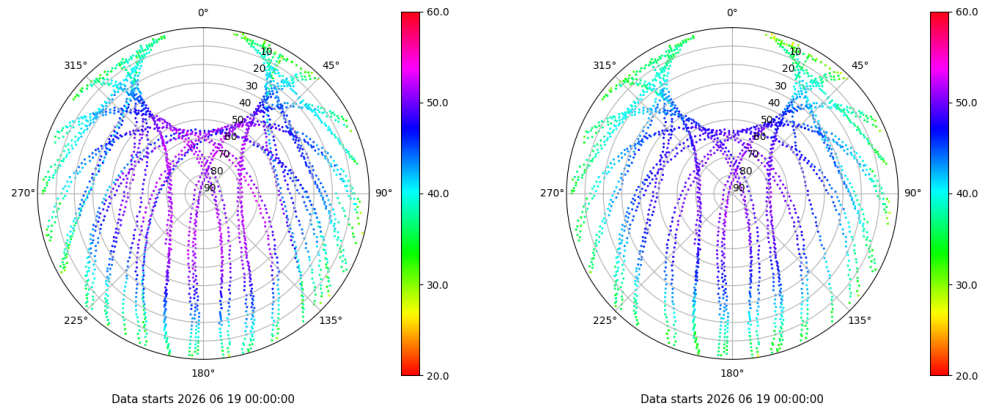
Skyplot for station VALC. Signal to Noise S1C Data file VALC00ESP_R_2026170.xtr Skyplot for station VALC. Signal to Noise S2C Data file VALC00ESP_R_2026170.xtr
