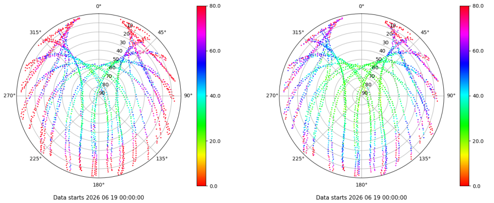
Skyplot for station VALC. Parameter M1C Data file VALC00ESP_R_2026170.xtr Skyplot for station VALC. Parameter M2C Data file VALC00ESP_R_2026170.xtr
