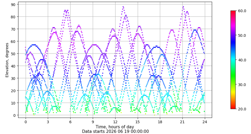
Time-elevation plot for station VALC. Signal to Noise S1C Data file VALC00ESP_R_2026170.xtr
