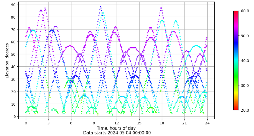
Time-elevation plot for station VALC. Signal to Noise S1C Data file VALC00ESP_R_2024125.xtr
