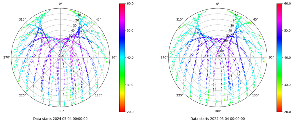
Skyplot for station VALC. Signal to Noise S1C Data file VALC00ESP_R_2024125.xtr Skyplot for station VALC. Signal to Noise S2C Data file VALC00ESP_R_2024125.xtr
