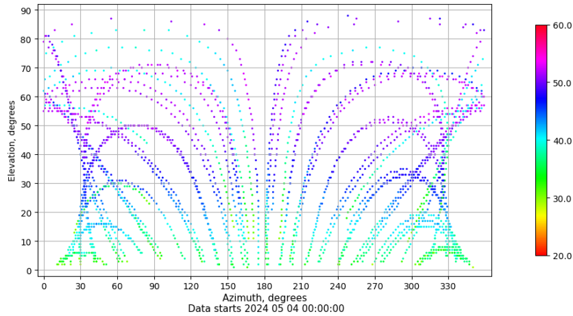
Azimuth-elevation plot for station VALC. Signal to Noise S1C Data file VALC00ESP_R_2024125.xtr
