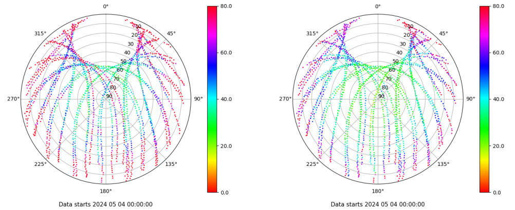
Skyplot for station VALC. Parameter M1C Data file VALC00ESP_R_2024125.xtr Skyplot for station VALC. Parameter M2C Data file VALC00ESP_R_2024125.xtr
