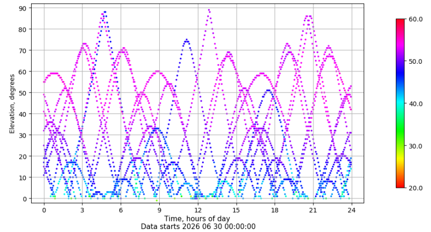
Time-elevation plot for station VALA. Signal to Noise S1C Data file VALA00ESP_R_2026181.xtr
