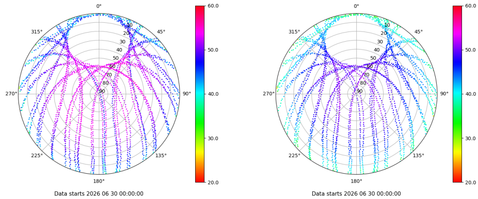
Skyplot for station VALA. Signal to Noise S1C Data file VALA00ESP_R_2026181.xtr Skyplot for station VALA. Signal to Noise S2C Data file VALA00ESP_R_2026181.xtr
