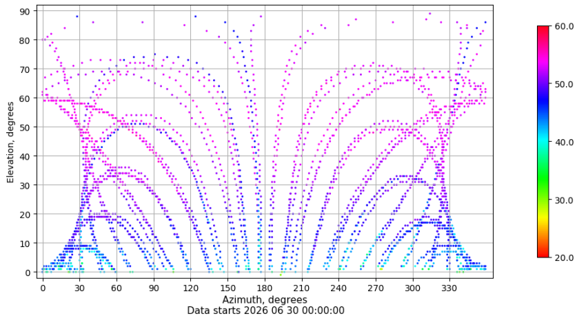
Azimuth-elevation plot for station VALA. Signal to Noise S1C Data file VALA00ESP_R_2026181.xtr
