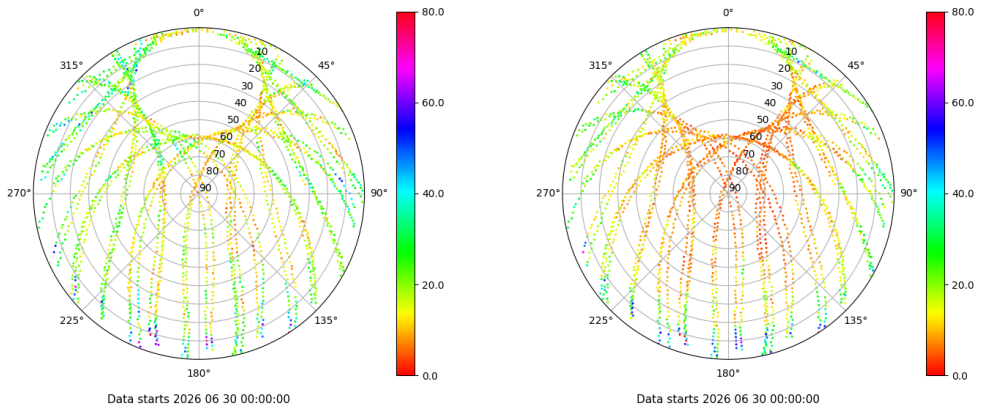
Skyplot for station VALA. Parameter M1C Data file VALA00ESP_R_2026181.xtr Skyplot for station VALA. Parameter M2C Data file VALA00ESP_R_2026181.xtr
