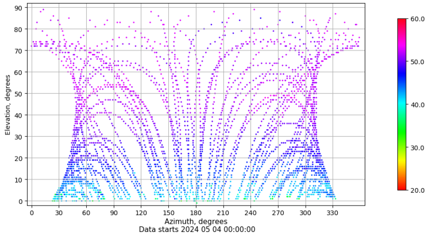
Azimuth-elevation plot for station VALA. Signal to Noise S1C Data file VALA00ESP_R_2024125.xtr
