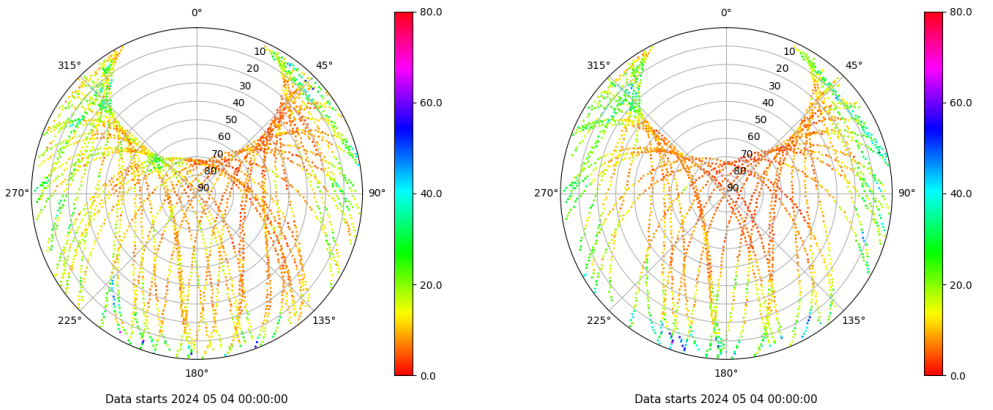
Skyplot for station VALA. Parameter M1C Data file VALA00ESP_R_2024125.xtr Skyplot for station VALA. Parameter M2S Data file VALA00ESP_R_2024125.xtr
