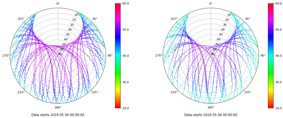
Skyplot for station VALA. Signal to Noise S1C Data file VALA00ESP_R_2024125.xtr Skyplot for station VALA. Signal to Noise S2S Data file VALA00ESP_R_2024125.xtr
