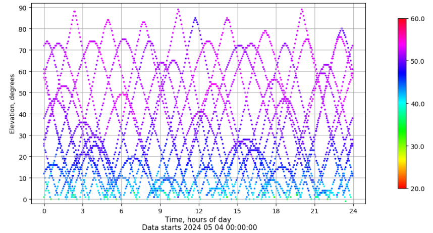
Time-elevation plot for station VALA. Signal to Noise S1C Data file VALA00ESP_R_2024125.xtr
