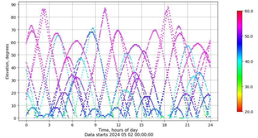
Time-elevation plot for station VALA. Signal to Noise S1C Data file VALA00ESP_R_2024123.xtr
