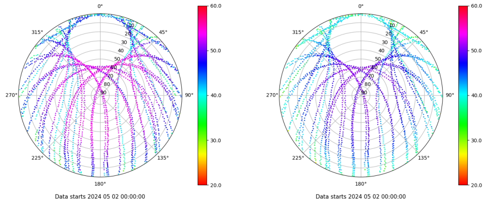
Skyplot for station VALA. Signal to Noise S1C Data file VALA00ESP_R_2024123.xtr Skyplot for station VALA. Signal to Noise S2C Data file VALA00ESP_R_2024123.xtr
