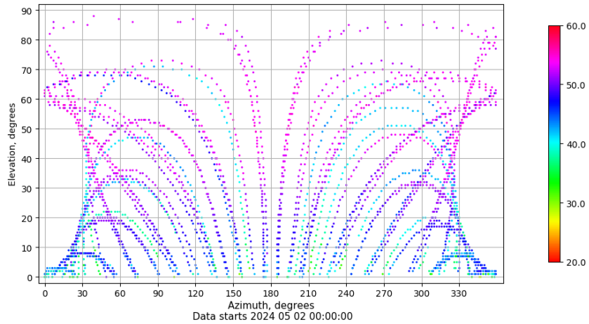
Azimuth-elevation plot for station VALA. Signal to Noise S1C Data file VALA00ESP_R_2024123.xtr
