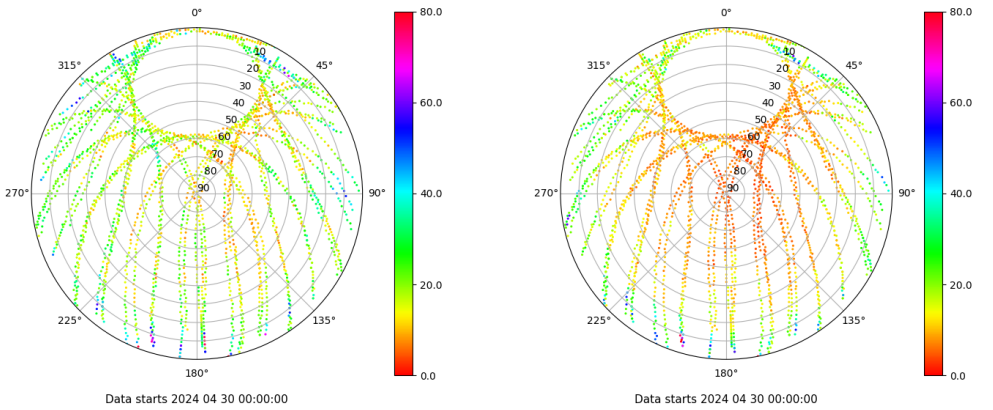
Skyplot for station VALA. Parameter M1C Data file VALA00ESP_R_2024121.xtr Skyplot for station VALA. Parameter M2C Data file VALA00ESP_R_2024121.xtr
