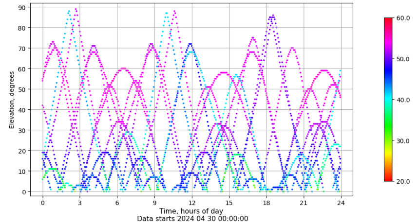
Time-elevation plot for station VALA. Signal to Noise S1C Data file VALA00ESP_R_2024121.xtr
