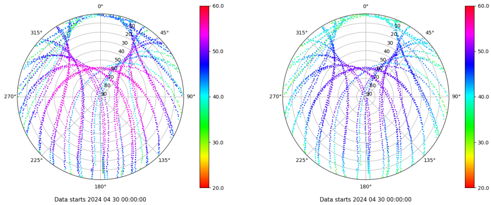
Skyplot for station VALA. Signal to Noise S1C Data file VALA00ESP_R_2024121.xtr Skyplot for station VALA. Signal to Noise S2C Data file VALA00ESP_R_2024121.xtr
