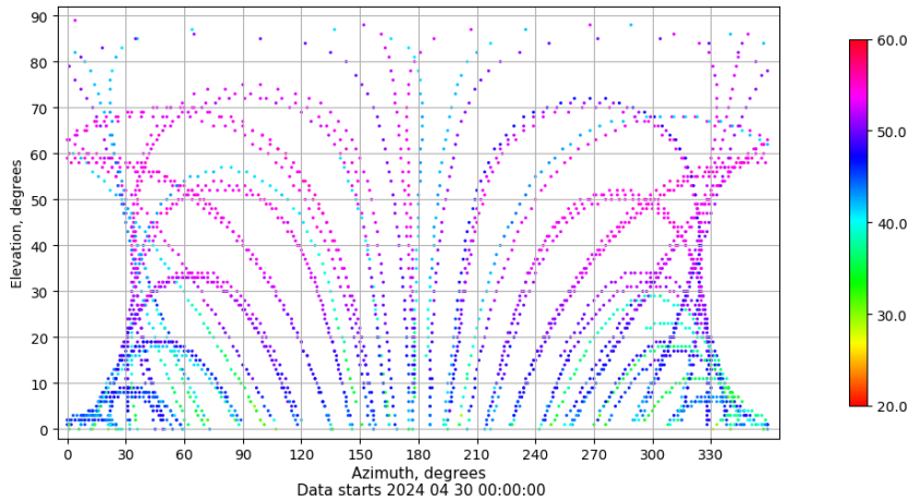
Azimuth-elevation plot for station VALA. Signal to Noise S1C Data file VALA00ESP_R_2024121.xtr
