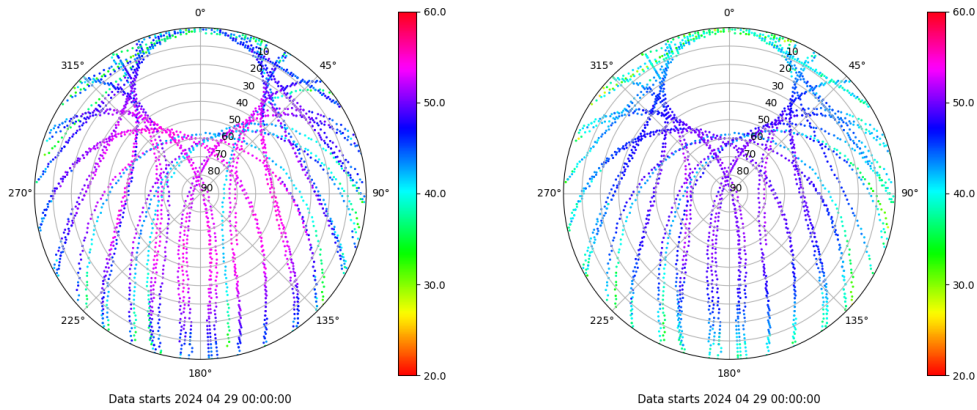
Skyplot for station VALA. Signal to Noise S1C Data file VALA00ESP_R_2024120.xtr Skyplot for station VALA. Signal to Noise S2C Data file VALA00ESP_R_2024120.xtr
