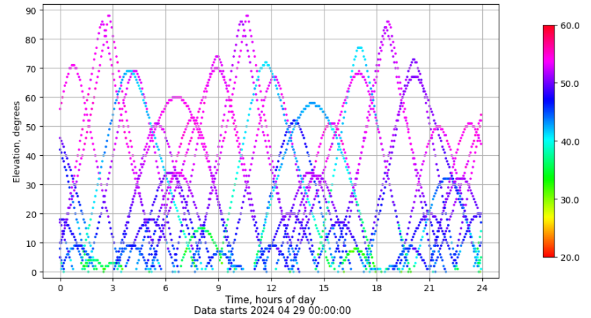
Time-elevation plot for station VALA. Signal to Noise S1C Data file VALA00ESP_R_2024120.xtr
