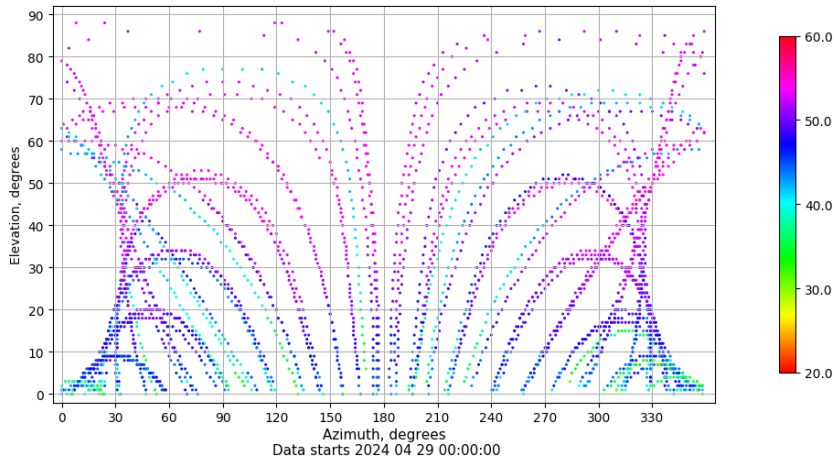
Azimuth-elevation plot for station VALA. Signal to Noise S1C Data file VALA00ESP_R_2024120.xtr
