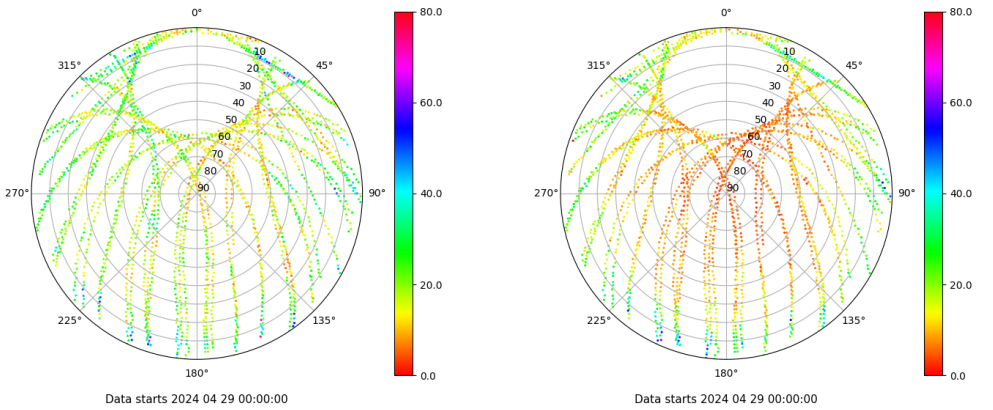
Skyplot for station VALA. Parameter M1C Data file VALA00ESP_R_2024120.xtr Skyplot for station VALA. Parameter M2C Data file VALA00ESP_R_2024120.xtr
