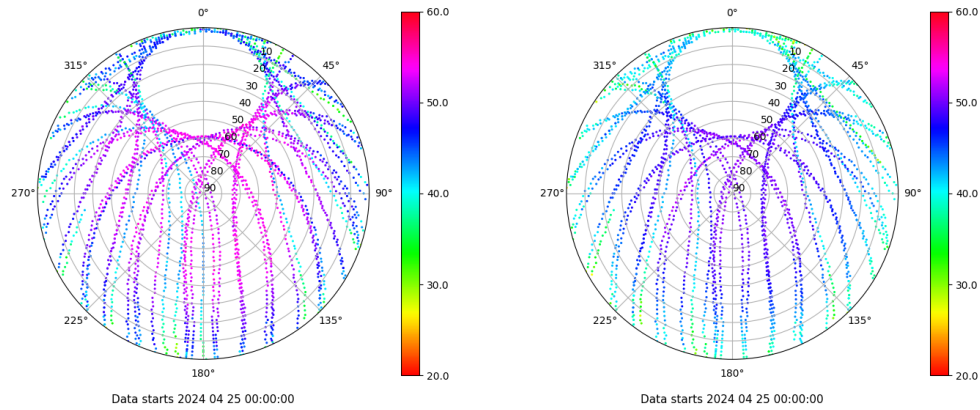
Skyplot for station VALA. Signal to Noise S1C Data file VALA00ESP_R_2024116.xtr Skyplot for station VALA. Signal to Noise S2C Data file VALA00ESP_R_2024116.xtr
