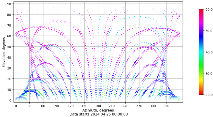
Azimuth-elevation plot for station VALA. Signal to Noise S1C Data file VALA00ESP_R_2024116.xtr
