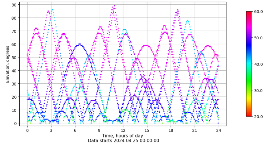
Time-elevation plot for station VALA. Signal to Noise S1C Data file VALA00ESP_R_2024116.xtr
