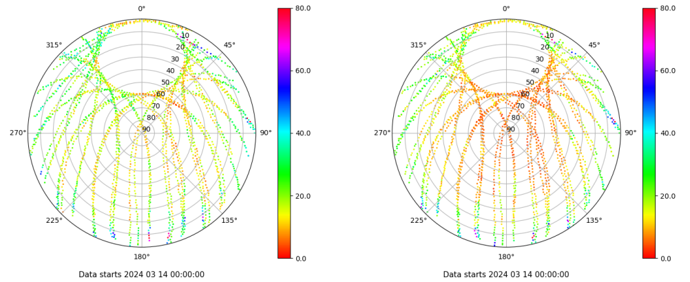
Skyplot for station VALA. Parameter M1C Data file VALA00ESP_R_2024074.xtr Skyplot for station VALA. Parameter M2C Data file VALA00ESP_R_2024074.xtr
