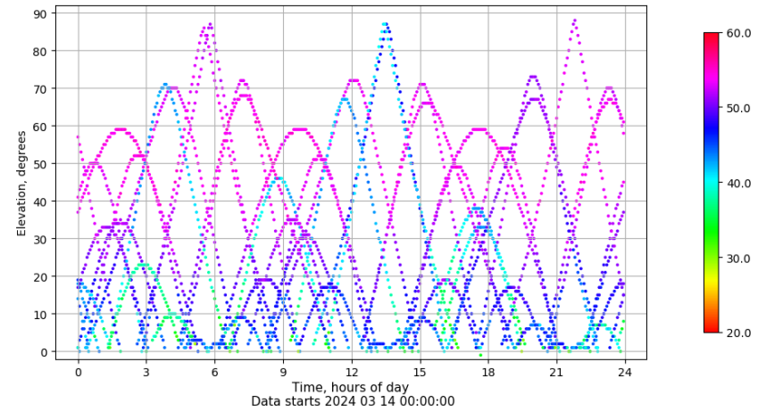
Time-elevation plot for station VALA. Signal to Noise S1C Data file VALA00ESP_R_2024074.xtr
