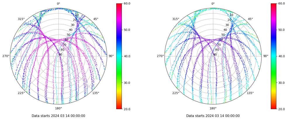
Skyplot for station VALA. Signal to Noise S1C Data file VALA00ESP_R_2024074.xtr Skyplot for station VALA. Signal to Noise S2C Data file VALA00ESP_R_2024074.xtr
