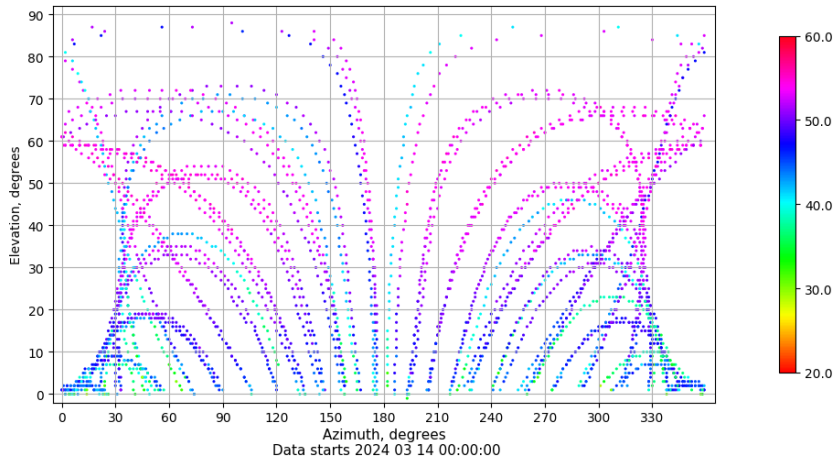
Azimuth-elevation plot for station VALA. Signal to Noise S1C Data file VALA00ESP_R_2024074.xtr
