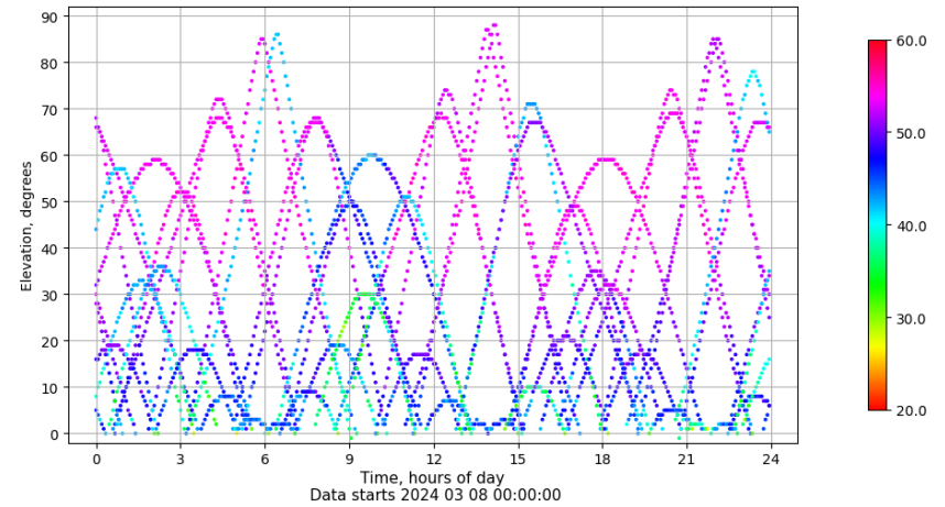
Time-elevation plot for station VALA. Signal to Noise S1C Data file VALA00ESP_R_2024068.xtr
