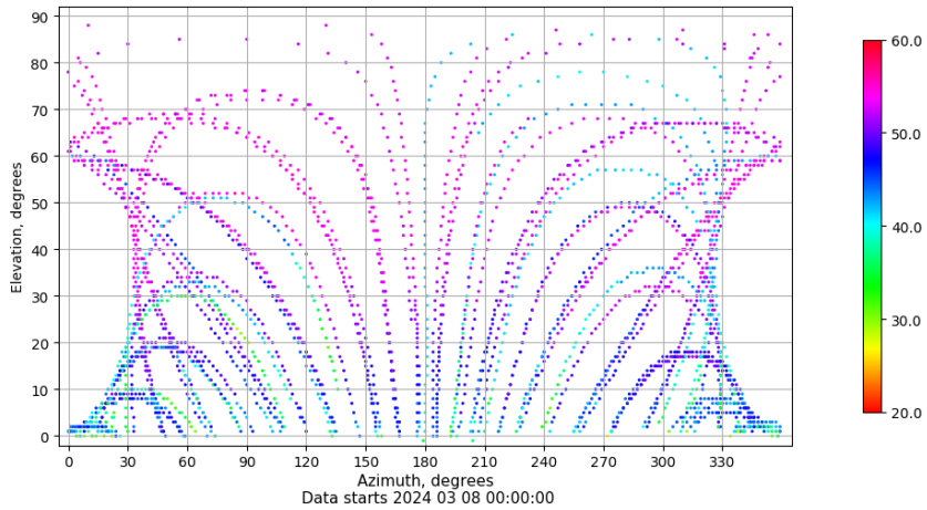
Azimuth-elevation plot for station VALA. Signal to Noise S1C Data file VALA00ESP_R_2024068.xtr
