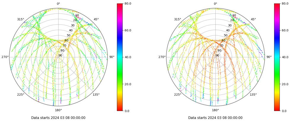
Skyplot for station VALA. Parameter M1C Data file VALA00ESP_R_2024068.xtr Skyplot for station VALA. Parameter M2C Data file VALA00ESP_R_2024068.xtr
