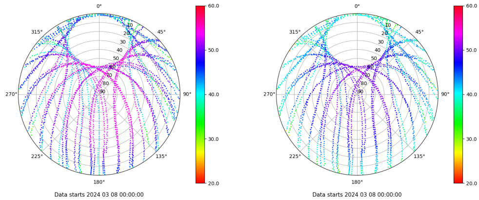
Skyplot for station VALA. Signal to Noise S1C Data file VALA00ESP_R_2024068.xtr Skyplot for station VALA. Signal to Noise S2C Data file VALA00ESP_R_2024068.xtr
