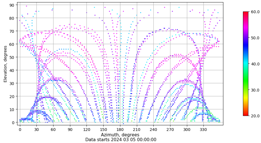
Azimuth-elevation plot for station VALA. Signal to Noise S1C Data file VALA00ESP_R_2024065.xtr
