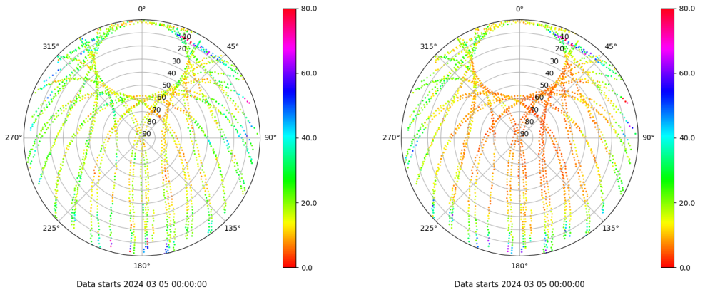
Skyplot for station VALA. Parameter M1C Data file VALA00ESP_R_2024065.xtr Skyplot for station VALA. Parameter M2C Data file VALA00ESP_R_2024065.xtr
