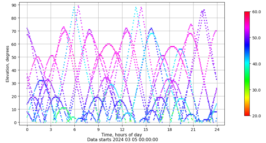
Time-elevation plot for station VALA. Signal to Noise S1C Data file VALA00ESP_R_2024065.xtr
