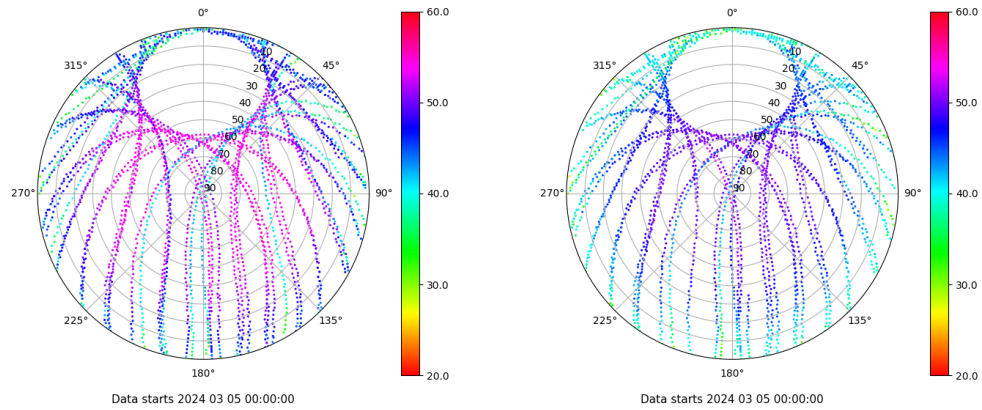
Skyplot for station VALA. Signal to Noise S1C Data file VALA00ESP_R_2024065.xtr Skyplot for station VALA. Signal to Noise S2C Data file VALA00ESP_R_2024065.xtr
