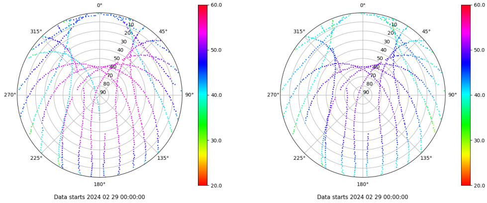
Skyplot for station VALA. Signal to Noise S1C Data file VALA00ESP_R_2024060.xtr Skyplot for station VALA. Signal to Noise S2C Data file VALA00ESP_R_2024060.xtr
