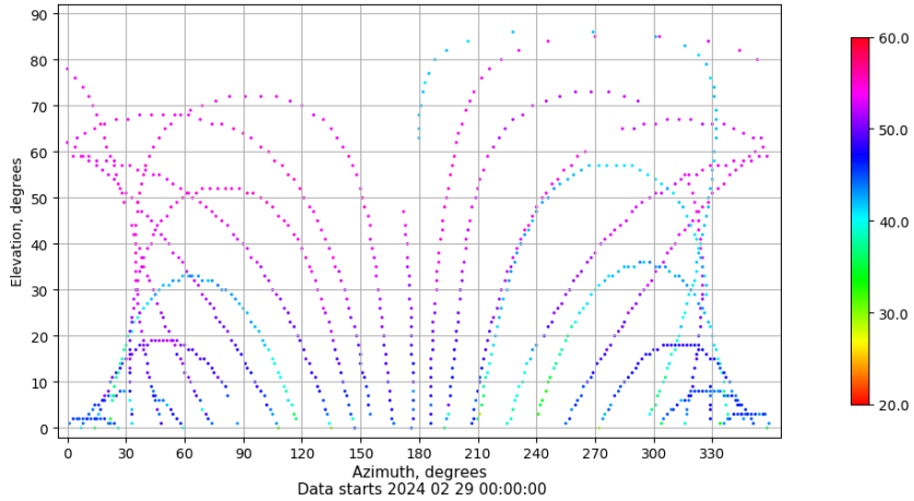
Azimuth-elevation plot for station VALA. Signal to Noise S1C Data file VALA00ESP_R_2024060.xtr
