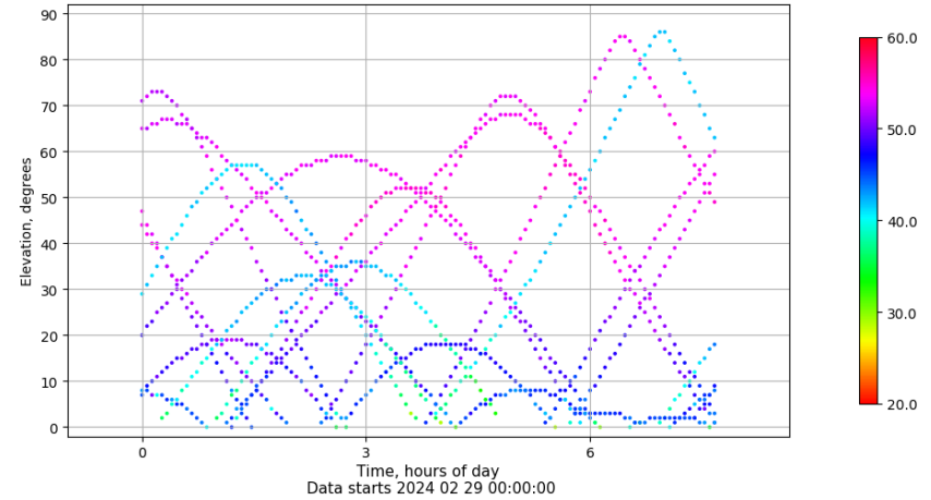
Time-elevation plot for station VALA. Signal to Noise S1C Data file VALA00ESP_R_2024060.xtr
