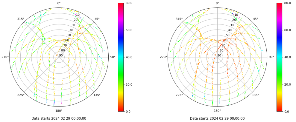
Skyplot for station VALA. Parameter M1C Data file VALA00ESP_R_2024060.xtr Skyplot for station VALA. Parameter M2C Data file VALA00ESP_R_2024060.xtr
