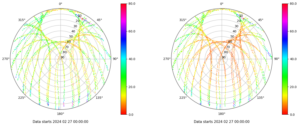
Skyplot for station VALA. Parameter M1C Data file VALA00ESP_R_2024058.xtr Skyplot for station VALA. Parameter M2C Data file VALA00ESP_R_2024058.xtr
