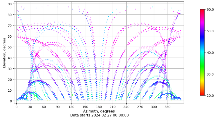
Azimuth-elevation plot for station VALA. Signal to Noise S1C Data file VALA00ESP_R_2024058.xtr
