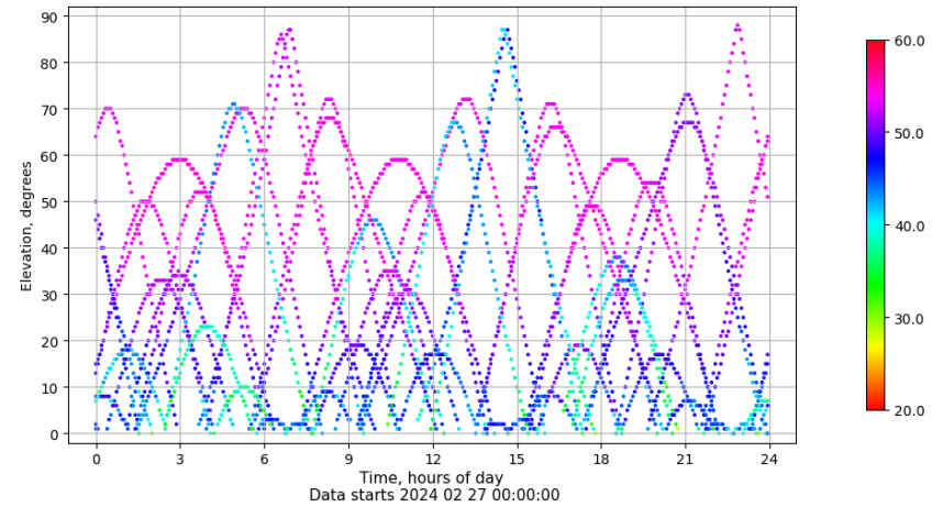
Time-elevation plot for station VALA. Signal to Noise S1C Data file VALA00ESP_R_2024058.xtr
