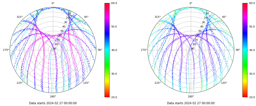
Skyplot for station VALA. Signal to Noise S1C Data file VALA00ESP_R_2024058.xtr Skyplot for station VALA. Signal to Noise S2C Data file VALA00ESP_R_2024058.xtr
