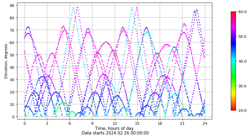
Time-elevation plot for station VALA. Signal to Noise S1C Data file VALA00ESP_R_2024057.xtr
