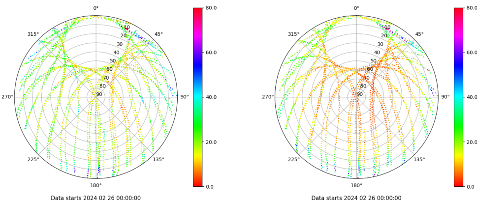
Skyplot for station VALA. Parameter M1C Data file VALA00ESP_R_2024057.xtr Skyplot for station VALA. Parameter M2C Data file VALA00ESP_R_2024057.xtr
