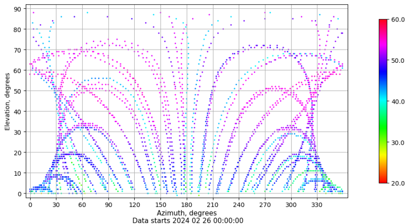
Azimuth-elevation plot for station VALA. Signal to Noise S1C Data file VALA00ESP_R_2024057.xtr
