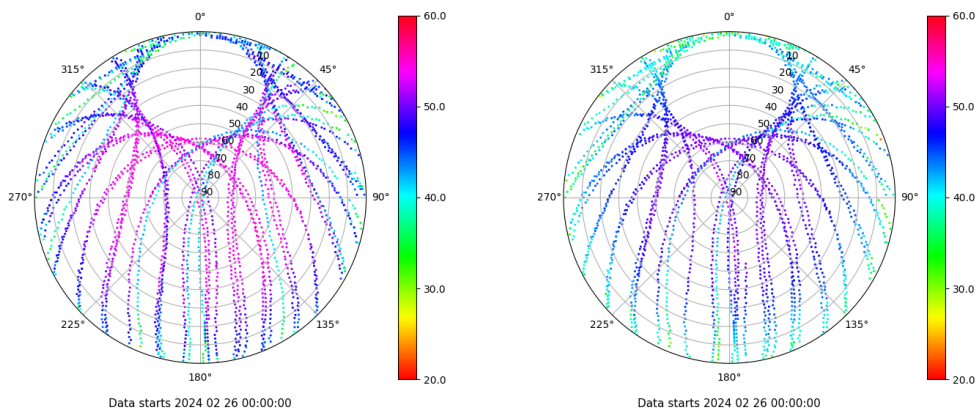
Skyplot for station VALA. Signal to Noise S1C Data file VALA00ESP_R_2024057.xtr Skyplot for station VALA. Signal to Noise S2C Data file VALA00ESP_R_2024057.xtr
