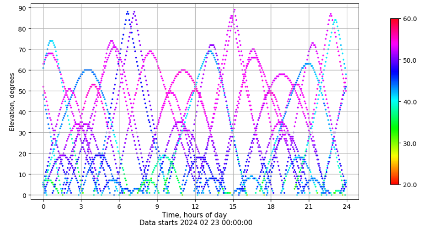
Time-elevation plot for station VALA. Signal to Noise S1C Data file VALA00ESP_R_2024054.xtr
