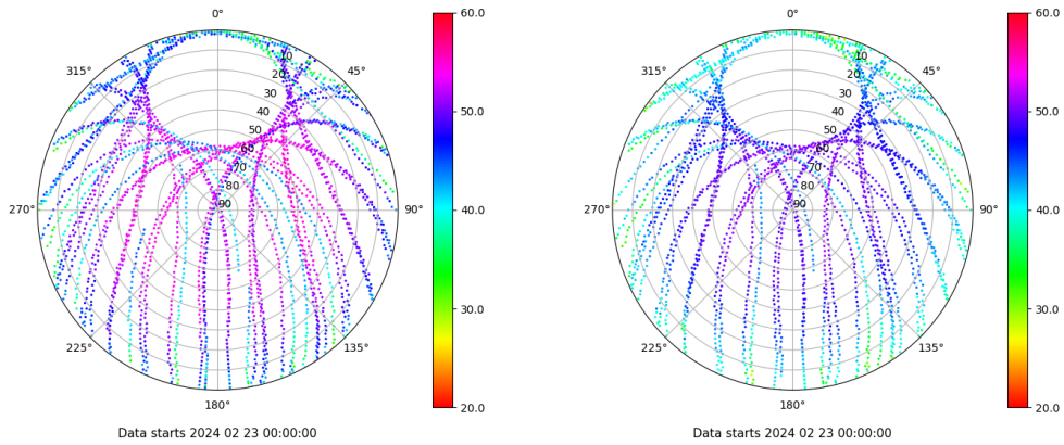
Skyplot for station VALA. Signal to Noise S1C Data file VALA00ESP_R_2024054.xtr Skyplot for station VALA. Signal to Noise S2C Data file VALA00ESP_R_2024054.xtr
