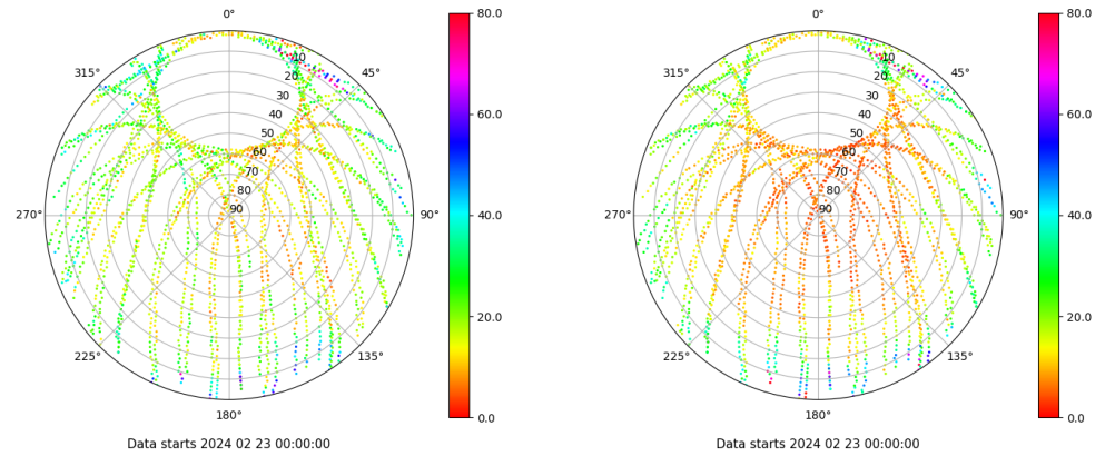
Skyplot for station VALA. Parameter M1C Data file VALA00ESP_R_2024054.xtr Skyplot for station VALA. Parameter M2C Data file VALA00ESP_R_2024054.xtr
