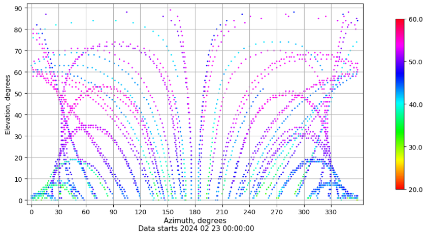
Azimuth-elevation plot for station VALA. Signal to Noise S1C Data file VALA00ESP_R_2024054.xtr
