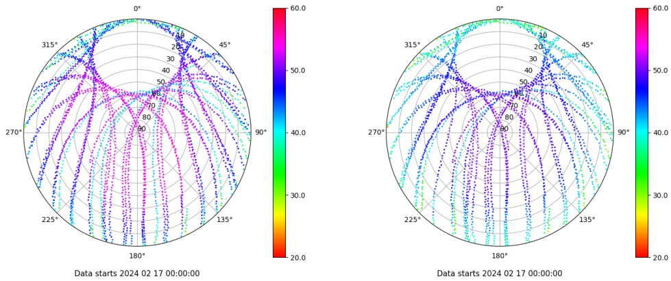
Skyplot for station VALA. Signal to Noise S1C Data file VALA00ESP_R_2024048.xtr Skyplot for station VALA. Signal to Noise S2C Data file VALA00ESP_R_2024048.xtr
