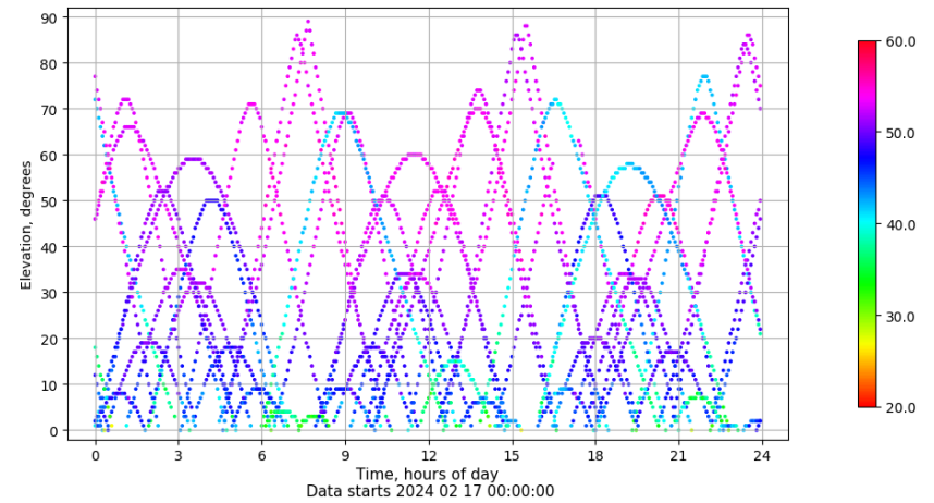
Time-elevation plot for station VALA. Signal to Noise S1C Data file VALA00ESP_R_2024048.xtr
