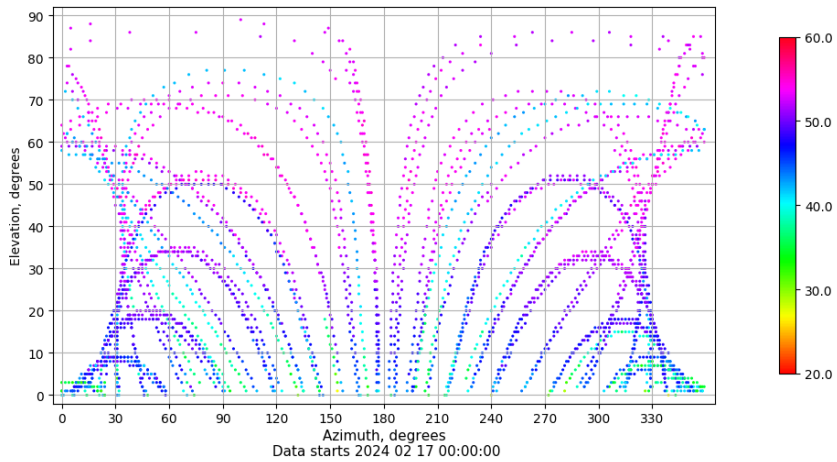
Azimuth-elevation plot for station VALA. Signal to Noise S1C Data file VALA00ESP_R_2024048.xtr
