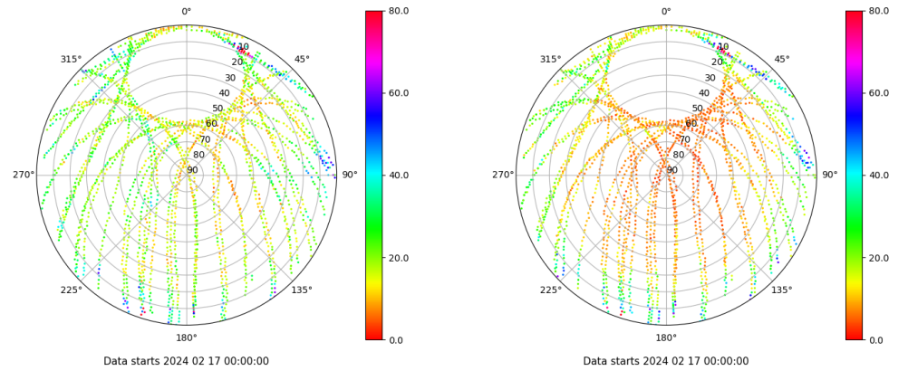
Skyplot for station VALA. Parameter M1C Data file VALA00ESP_R_2024048.xtr Skyplot for station VALA. Parameter M2C Data file VALA00ESP_R_2024048.xtr
