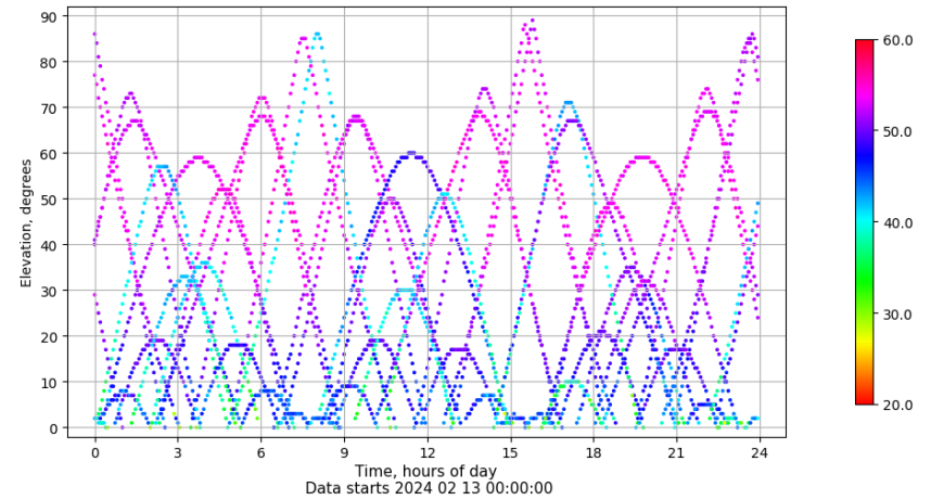
Time-elevation plot for station VALA. Signal to Noise S1C Data file VALA00ESP_R_2024044.xtr
