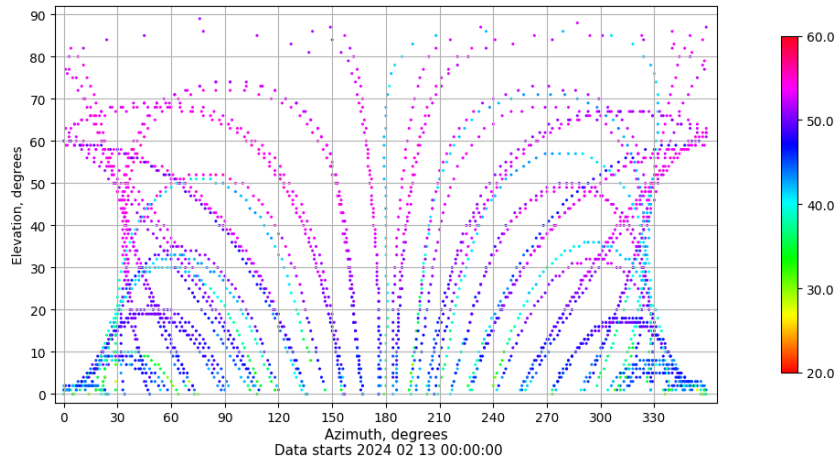
Azimuth-elevation plot for station VALA. Signal to Noise S1C Data file VALA00ESP_R_2024044.xtr
