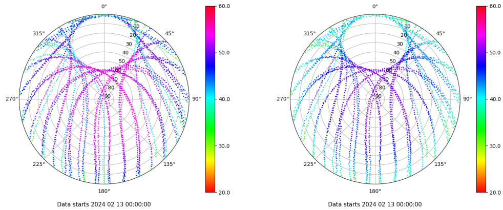
Skyplot for station VALA. Signal to Noise S1C Data file VALA00ESP_R_2024044.xtr Skyplot for station VALA. Signal to Noise S2C Data file VALA00ESP_R_2024044.xtr
