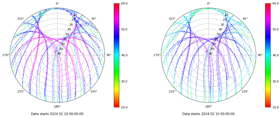
Skyplot for station VALA. Signal to Noise S1C Data file VALA00ESP_R_2024041.xtr Skyplot for station VALA. Signal to Noise S2C Data file VALA00ESP_R_2024041.xtr
