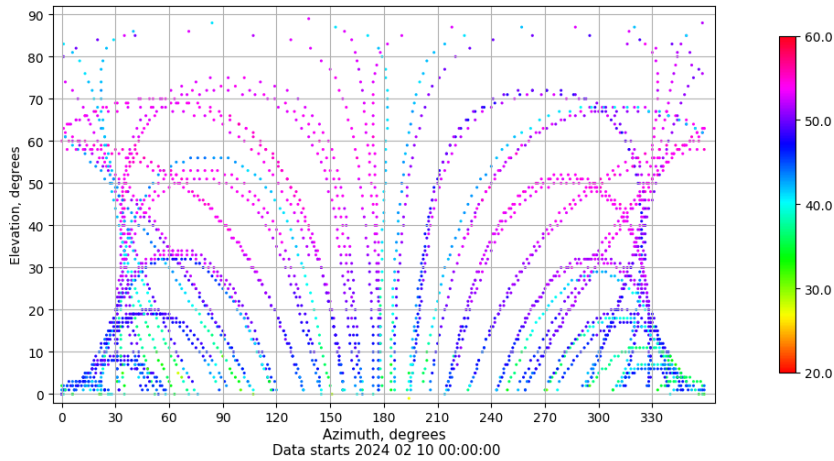
Azimuth-elevation plot for station VALA. Signal to Noise S1C Data file VALA00ESP_R_2024041.xtr
