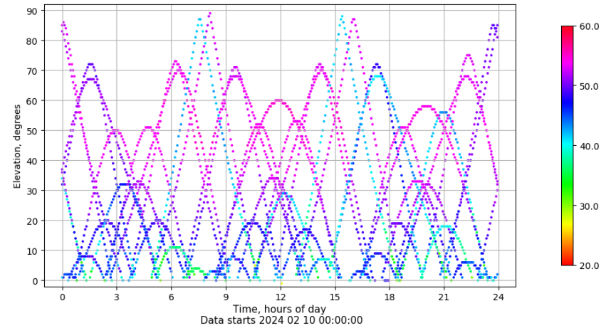
Time-elevation plot for station VALA. Signal to Noise S1C Data file VALA00ESP_R_2024041.xtr
