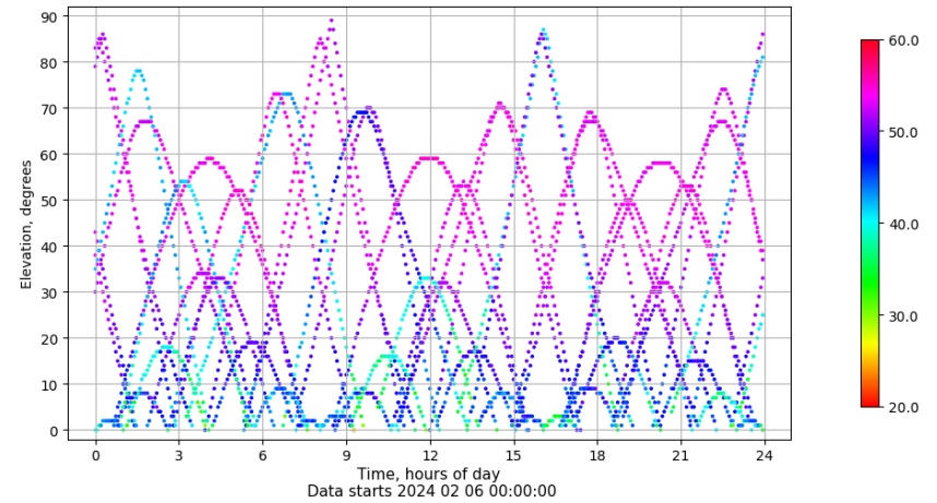
Time-elevation plot for station VALA. Signal to Noise S1C Data file VALA00ESP_R_2024037.xtr
