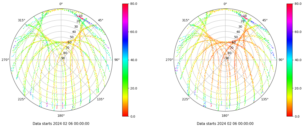
Skyplot for station VALA. Parameter M1C Data file VALA00ESP_R_2024037.xtr Skyplot for station VALA. Parameter M2C Data file VALA00ESP_R_2024037.xtr
