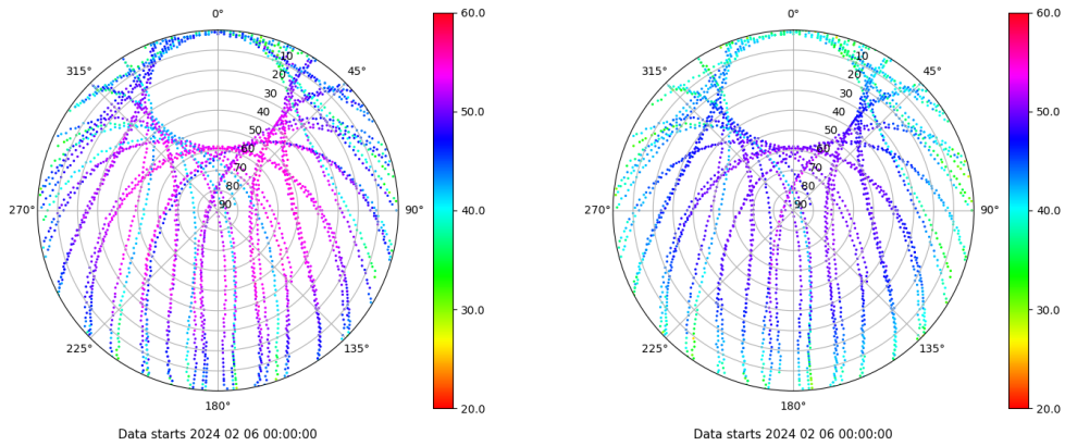
Skyplot for station VALA. Signal to Noise S1C Data file VALA00ESP_R_2024037.xtr Skyplot for station VALA. Signal to Noise S2C Data file VALA00ESP_R_2024037.xtr
