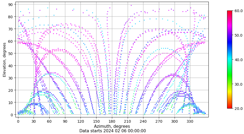
Azimuth-elevation plot for station VALA. Signal to Noise S1C Data file VALA00ESP_R_2024037.xtr
