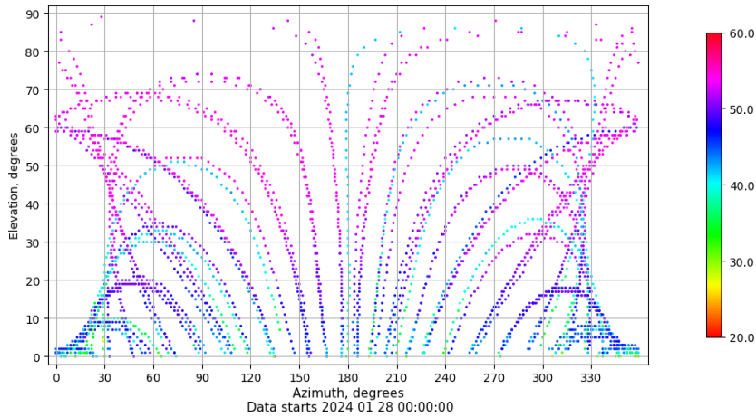
Azimuth-elevation plot for station VALA. Signal to Noise S1C Data file VALA00ESP_R_2024028.xtr
