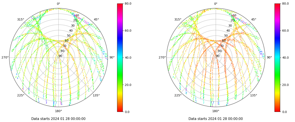
Skyplot for station VALA. Parameter M1C Data file VALA00ESP_R_2024028.xtr Skyplot for station VALA. Parameter M2C Data file VALA00ESP_R_2024028.xtr
