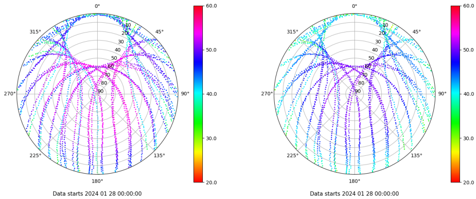
Skyplot for station VALA. Signal to Noise S1C Data file VALA00ESP_R_2024028.xtr Skyplot for station VALA. Signal to Noise S2C Data file VALA00ESP_R_2024028.xtr
