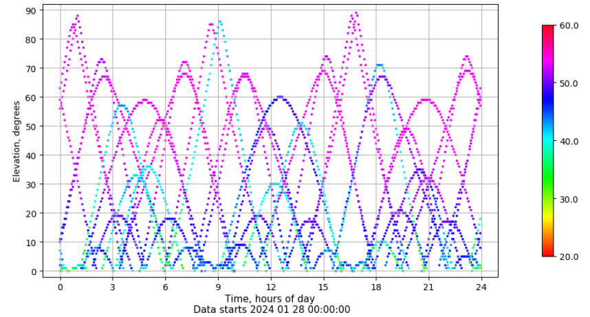
Time-elevation plot for station VALA. Signal to Noise S1C Data file VALA00ESP_R_2024028.xtr
