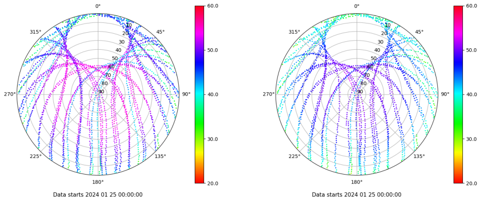
Skyplot for station VALA. Signal to Noise S1C Data file VALA00ESP_R_2024025.xtr Skyplot for station VALA. Signal to Noise S2C Data file VALA00ESP_R_2024025.xtr
