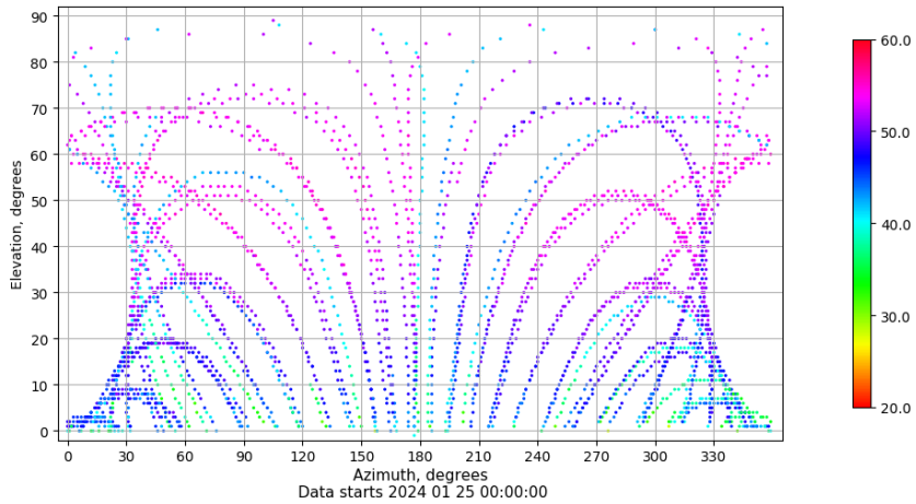
Azimuth-elevation plot for station VALA. Signal to Noise S1C Data file VALA00ESP_R_2024025.xtr
