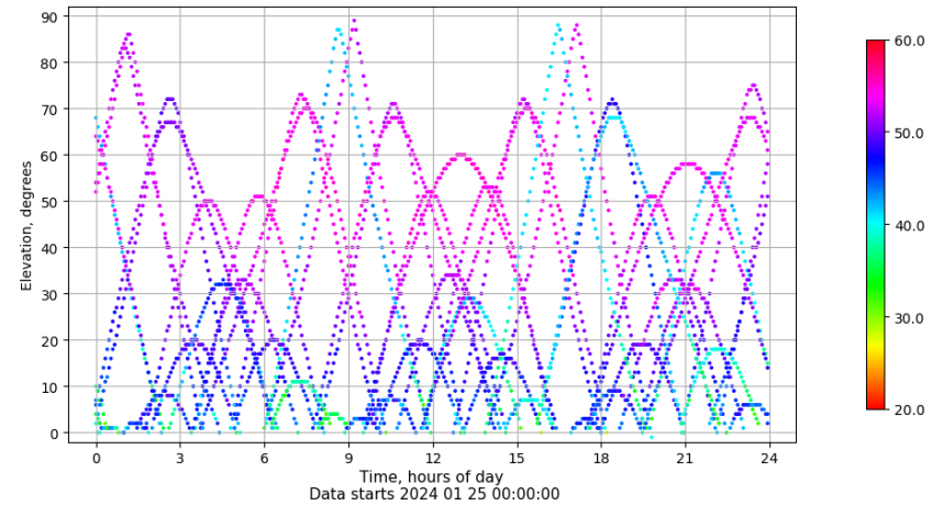
Time-elevation plot for station VALA. Signal to Noise S1C Data file VALA00ESP_R_2024025.xtr
