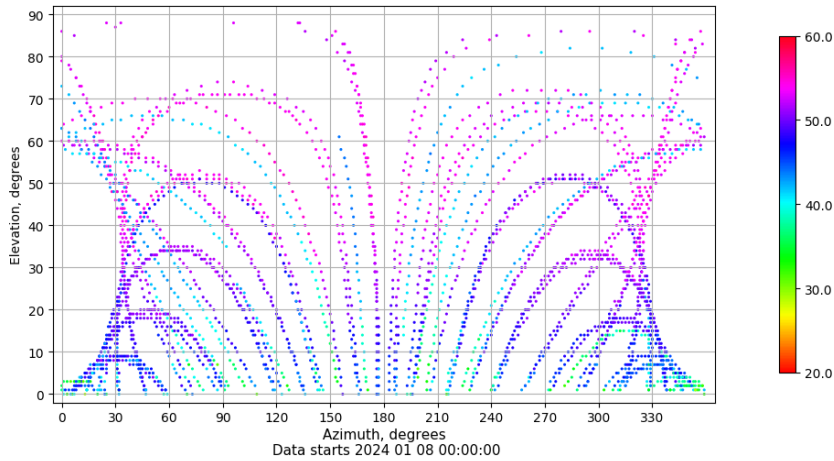
Azimuth-elevation plot for station VALA. Signal to Noise S1C Data file VALA00ESP_R_2024008.xtr
