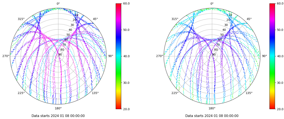
Skyplot for station VALA. Signal to Noise S1C Data file VALA00ESP_R_2024008.xtr Skyplot for station VALA. Signal to Noise S2C Data file VALA00ESP_R_2024008.xtr
