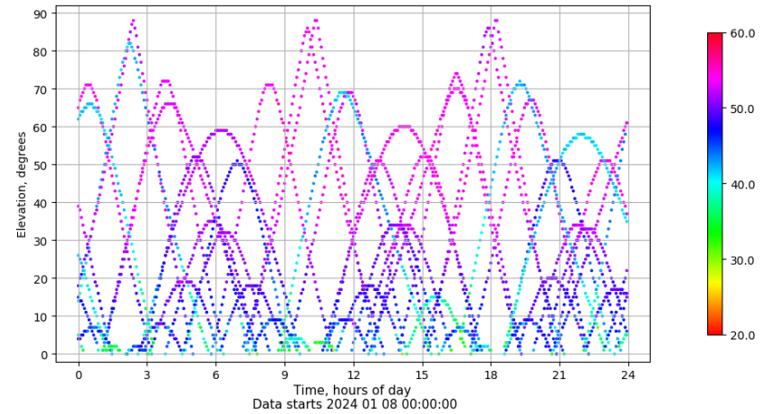
Time-elevation plot for station VALA. Signal to Noise S1C Data file VALA00ESP_R_2024008.xtr
