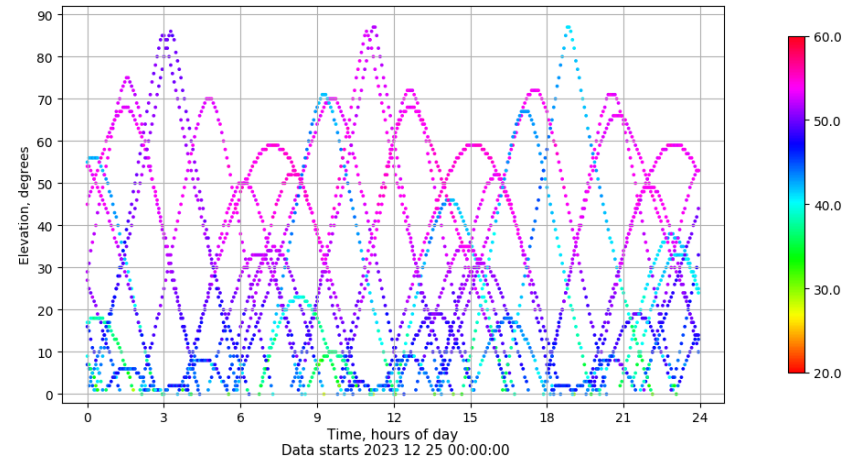
Time-elevation plot for station VALA. Signal to Noise S1C Data file VALA00ESP_R_2023359.xtr
