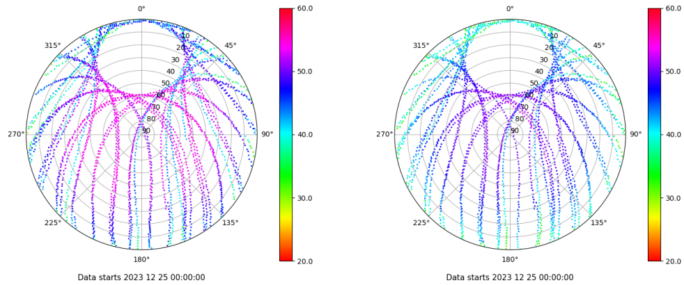
Skyplot for station VALA. Signal to Noise S1C Data file VALA00ESP_R_2023359.xtr Skyplot for station VALA. Signal to Noise S2C Data file VALA00ESP_R_2023359.xtr
