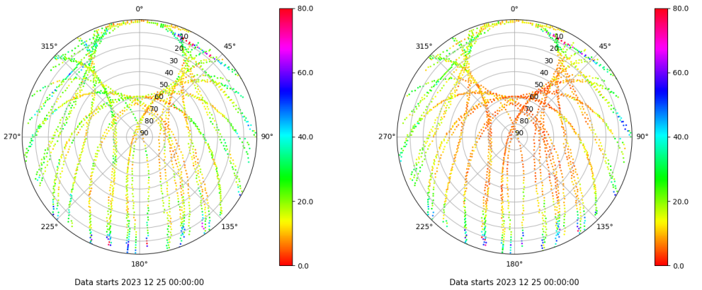
Skyplot for station VALA. Parameter M1C Data file VALA00ESP_R_2023359.xtr Skyplot for station VALA. Parameter M2C Data file VALA00ESP_R_2023359.xtr
