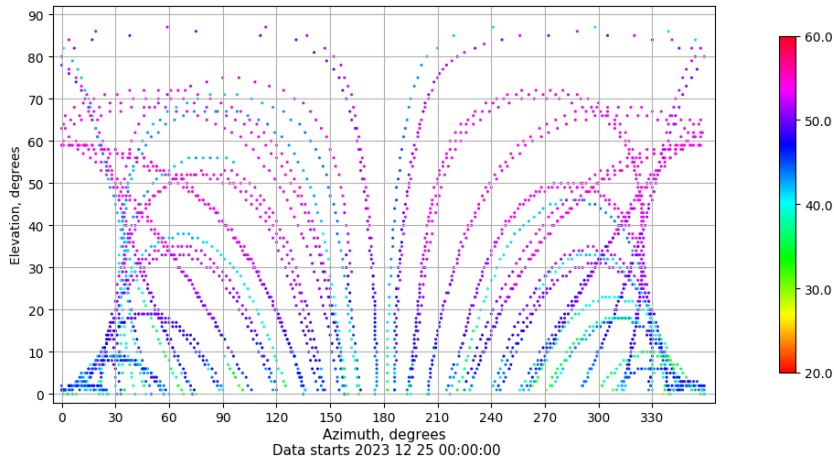
Azimuth-elevation plot for station VALA. Signal to Noise S1C Data file VALA00ESP_R_2023359.xtr
