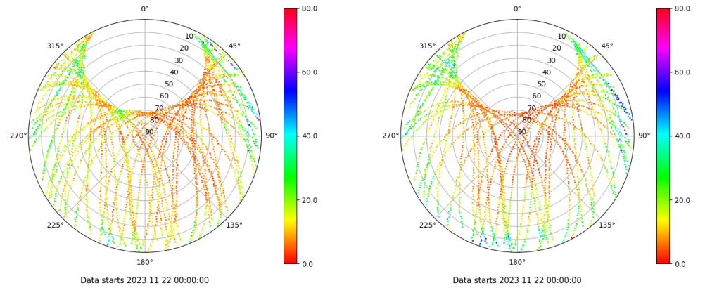
Skyplot for station VALA. Parameter M1C Data file VALA00ESP_R_2023326.xtr Skyplot for station VALA. Parameter M2S Data file VALA00ESP_R_2023326.xtr
