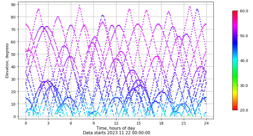
Time-elevation plot for station VALA. Signal to Noise S1C Data file VALA00ESP_R_2023326.xtr
