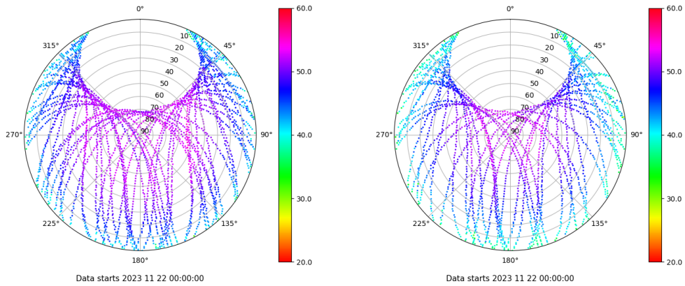
Skyplot for station VALA. Signal to Noise S1C Data file VALA00ESP_R_2023326.xtr Skyplot for station VALA. Signal to Noise S2S Data file VALA00ESP_R_2023326.xtr
