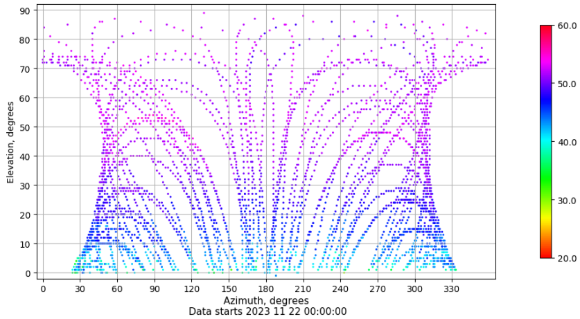
Azimuth-elevation plot for station VALA. Signal to Noise S1C Data file VALA00ESP_R_2023326.xtr
