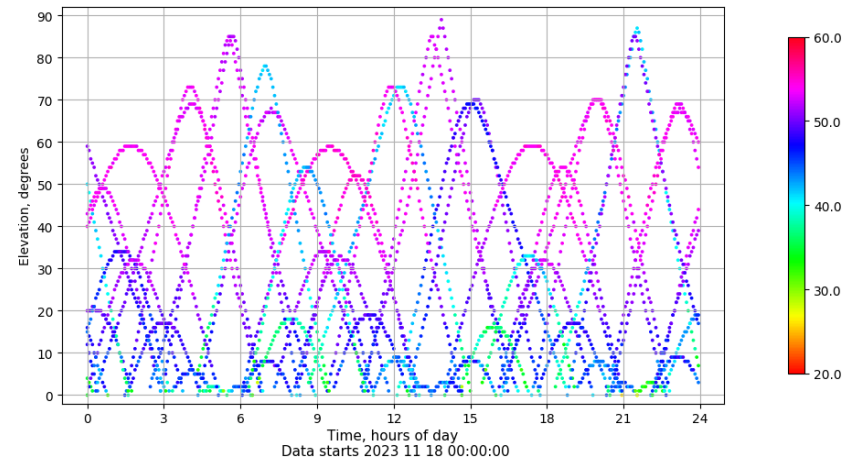
Time-elevation plot for station VALA. Signal to Noise S1C Data file VALA00ESP_R_2023322.xtr
