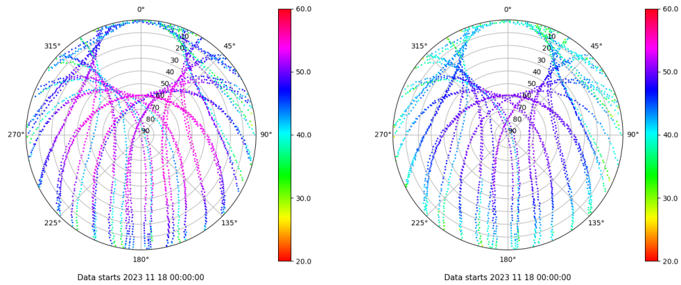
Skyplot for station VALA. Signal to Noise S1C Data file VALA00ESP_R_2023322.xtr Skyplot for station VALA. Signal to Noise S2C Data file VALA00ESP_R_2023322.xtr
