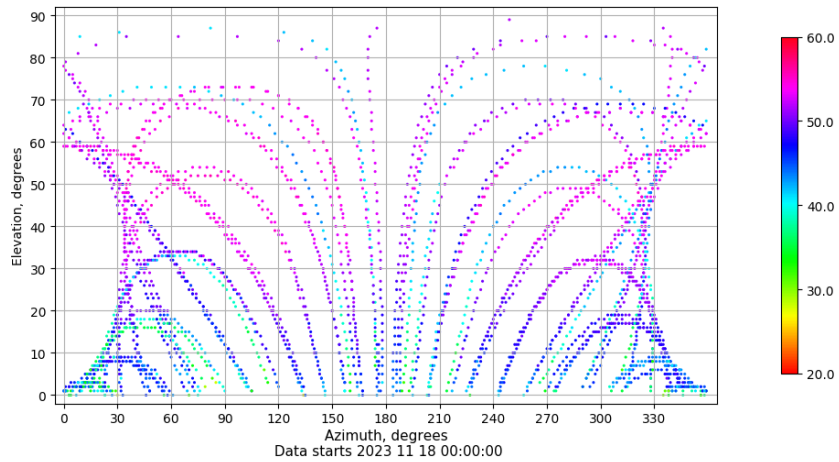
Azimuth-elevation plot for station VALA. Signal to Noise S1C Data file VALA00ESP_R_2023322.xtr
