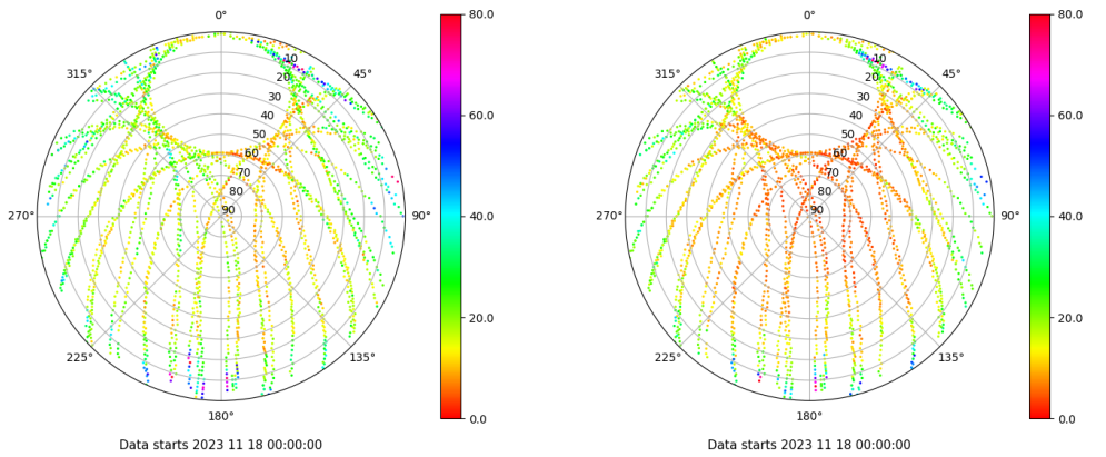
Skyplot for station VALA. Parameter M1C Data file VALA00ESP_R_2023322.xtr Skyplot for station VALA. Parameter M2C Data file VALA00ESP_R_2023322.xtr
