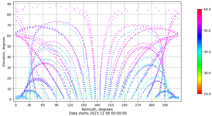
Azimuth-elevation plot for station VALA. Signal to Noise S1C Data file VALA00ESP_R_2023312.xtr
