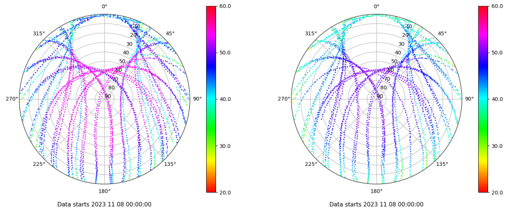
Skyplot for station VALA. Signal to Noise S1C Data file VALA00ESP_R_2023312.xtr Skyplot for station VALA. Signal to Noise S2C Data file VALA00ESP_R_2023312.xtr
