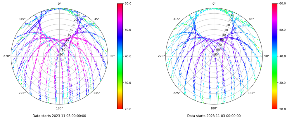
Skyplot for station VALA. Signal to Noise S1C Data file VALA00ESP_R_2023307.xtr Skyplot for station VALA. Signal to Noise S2C Data file VALA00ESP_R_2023307.xtr
