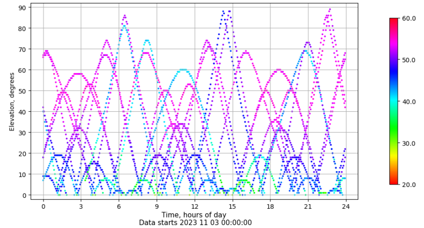
Time-elevation plot for station VALA. Signal to Noise S1C Data file VALA00ESP_R_2023307.xtr
