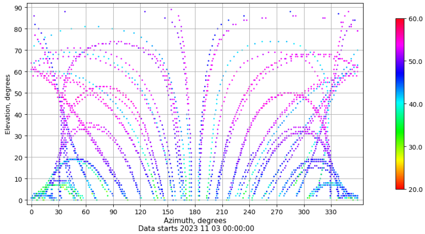
Azimuth-elevation plot for station VALA. Signal to Noise S1C Data file VALA00ESP_R_2023307.xtr
