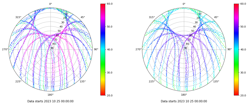
Skyplot for station VALA. Signal to Noise S1C Data file VALA00ESP_R_2023298.xtr Skyplot for station VALA. Signal to Noise S2C Data file VALA00ESP_R_2023298.xtr
