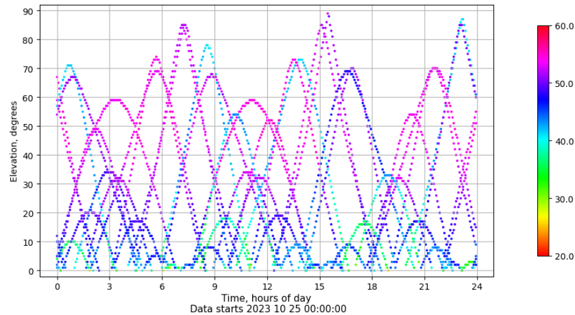
Time-elevation plot for station VALA. Signal to Noise S1C Data file VALA00ESP_R_2023298.xtr
