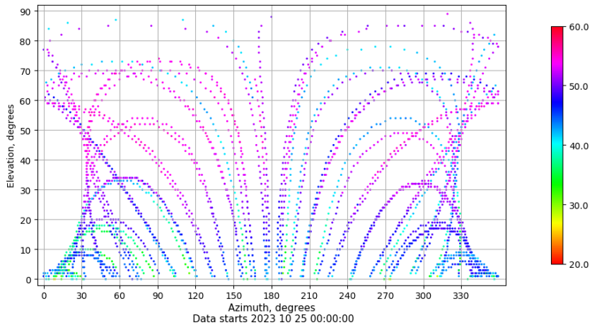
Azimuth-elevation plot for station VALA. Signal to Noise S1C Data file VALA00ESP_R_2023298.xtr
