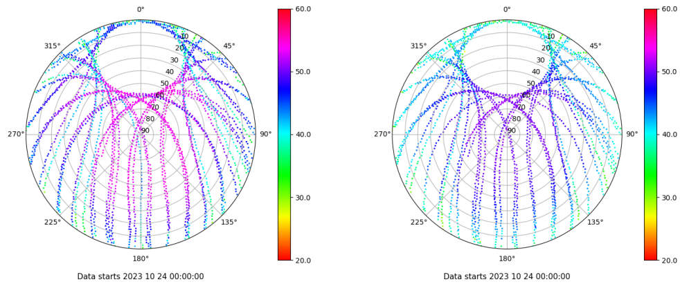
Skyplot for station VALA. Signal to Noise S1C Data file VALA00ESP_R_2023297.xtr Skyplot for station VALA. Signal to Noise S2C Data file VALA00ESP_R_2023297.xtr
