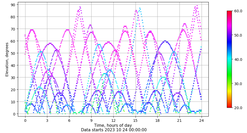
Time-elevation plot for station VALA. Signal to Noise S1C Data file VALA00ESP_R_2023297.xtr
