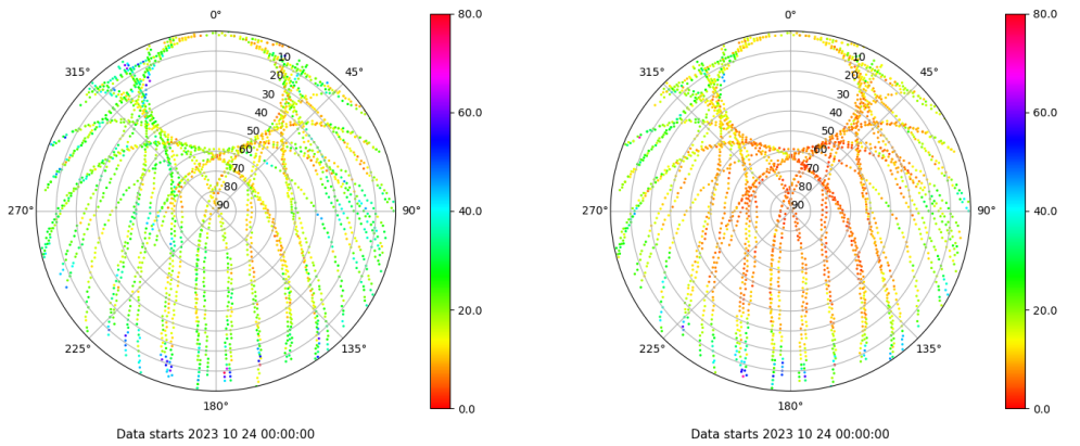
Skyplot for station VALA. Parameter M1C Data file VALA00ESP_R_2023297.xtr Skyplot for station VALA. Parameter M2C Data file VALA00ESP_R_2023297.xtr
