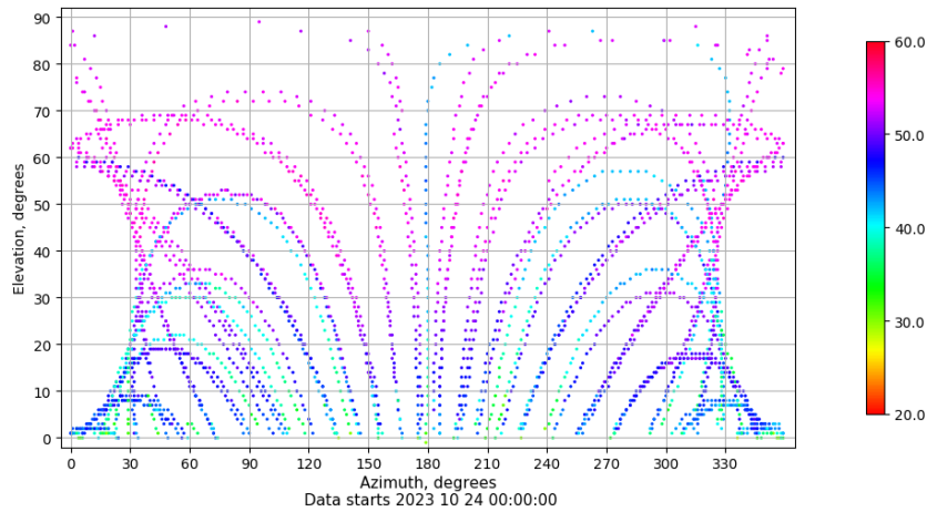
Azimuth-elevation plot for station VALA. Signal to Noise S1C Data file VALA00ESP_R_2023297.xtr
