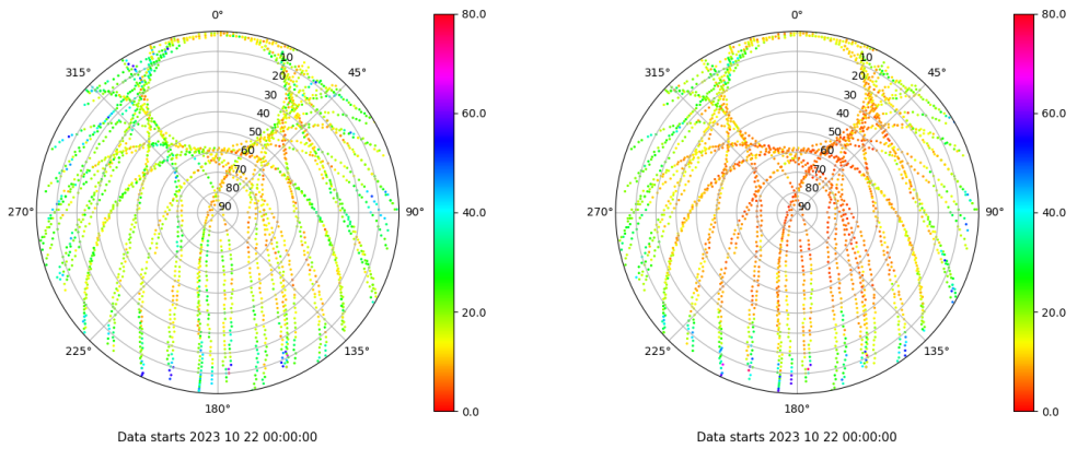
Skyplot for station VALA. Parameter M1C Data file VALA00ESP_R_2023295.xtr Skyplot for station VALA. Parameter M2C Data file VALA00ESP_R_2023295.xtr
