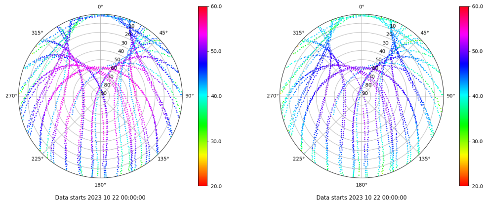
Skyplot for station VALA. Signal to Noise S1C Data file VALA00ESP_R_2023295.xtr Skyplot for station VALA. Signal to Noise S2C Data file VALA00ESP_R_2023295.xtr
