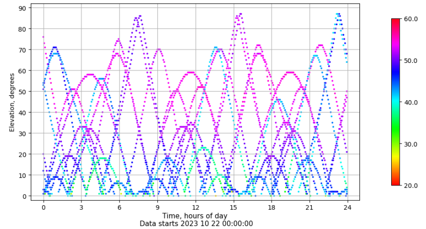
Time-elevation plot for station VALA. Signal to Noise S1C Data file VALA00ESP_R_2023295.xtr
