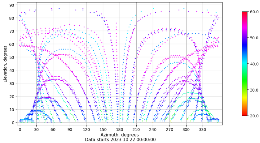
Azimuth-elevation plot for station VALA. Signal to Noise S1C Data file VALA00ESP_R_2023295.xtr
