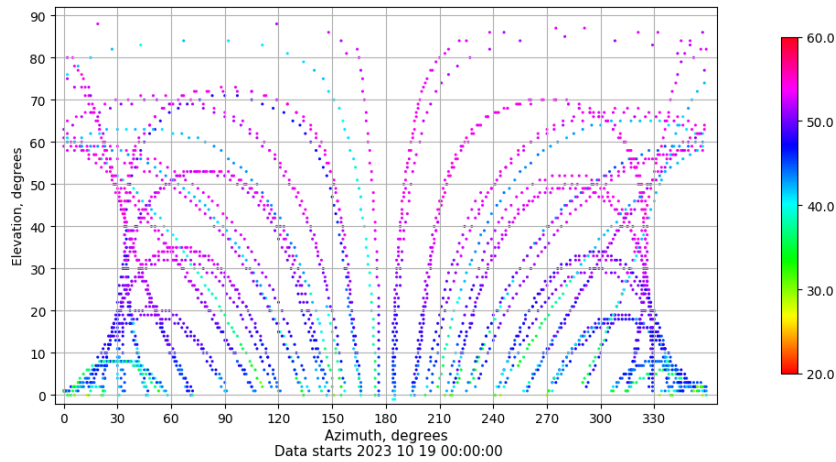
Azimuth-elevation plot for station VALA. Signal to Noise S1C Data file VALA00ESP_R_2023292.xtr
