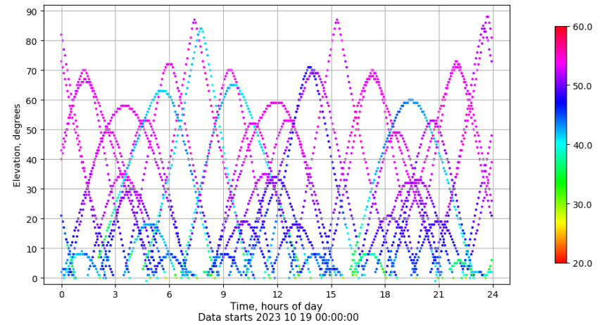
Time-elevation plot for station VALA. Signal to Noise S1C Data file VALA00ESP_R_2023292.xtr
