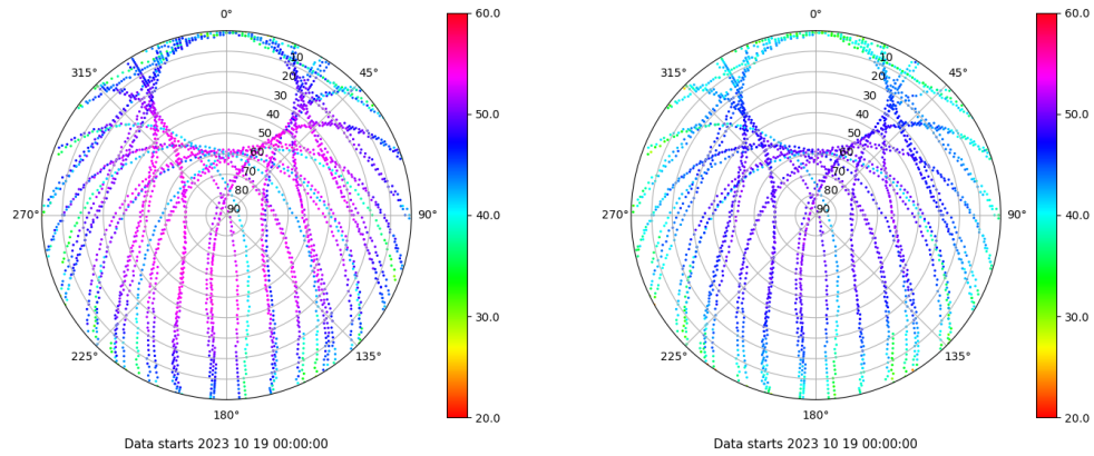
Skyplot for station VALA. Signal to Noise S1C Data file VALA00ESP_R_2023292.xtr Skyplot for station VALA. Signal to Noise S2C Data file VALA00ESP_R_2023292.xtr
