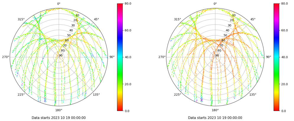
Skyplot for station VALA. Parameter M1C Data file VALA00ESP_R_2023292.xtr Skyplot for station VALA. Parameter M2C Data file VALA00ESP_R_2023292.xtr
